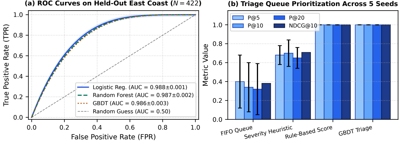
Fig. 3. (a) ROC curves with standard deviation bands across 5 independent seeds evaluated on the held-out East Coast partition ( N = 422 ), highlighting overlapping classifier performance; (b) Queue prioritization ranking metrics ( P@5 , P@10 , P@20 , NDCG@10 ), demonstrating that heuristic rules and GBDT triage significantly outperform FIFO and severity heuristics while matching each other on the synthetic benchmark.
