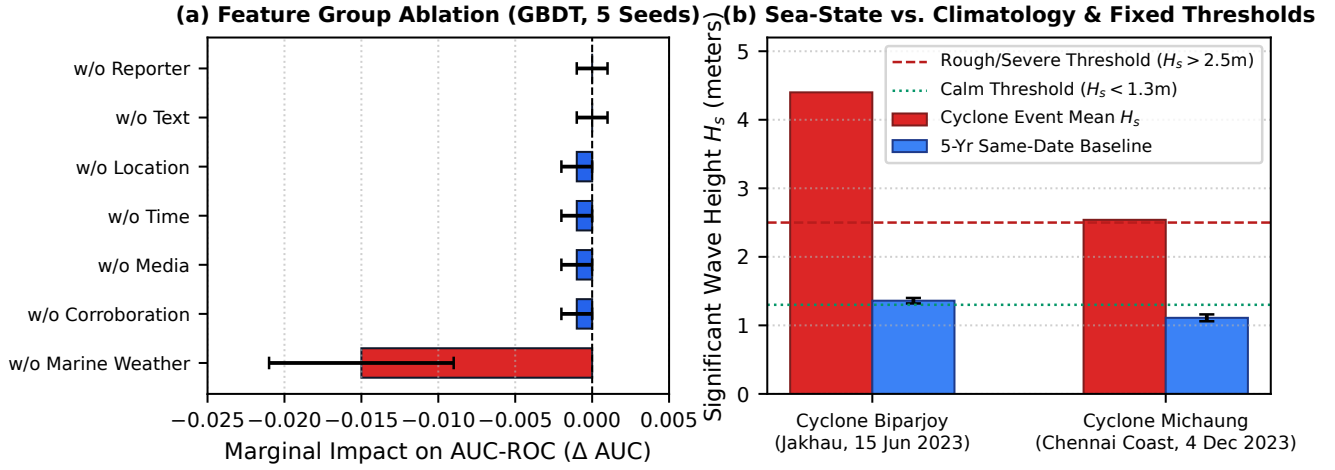
Fig. 4. (a) Feature group ablation study (GBDT, 5 seeds) showing marginal impact ( \Delta AUC) relative to the full 19-dimensional feature representation; (b) Physical grounding analysis comparing significant wave heights ( H_s ) during Cyclones Biparjoy and Michaung against 5-year same-date baselines and calm/severe thresholds, illustrating regional monsoon seasonality at Jakhau in June.
