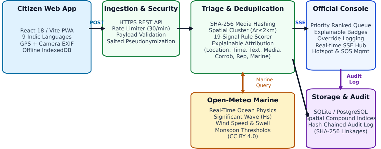
Fig. 1. Three-tier architecture of the OceanSaksham platform, showing citizen ingestion with EXIF/GPS telemetry, token-bucket rate limiting, spatial deduplication, real-time Open-Meteo marine sea-state validation, 19-signal explainable heuristic triage, SSE live event broadcasting, and append-only cryptographic hash-chained audit logging.
