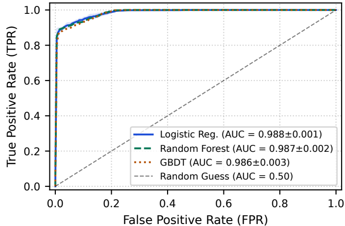
(a) Empirical ROC Curves Across 5 Seeds ( N = 422 )
