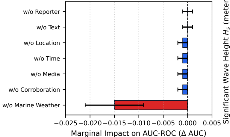
(a) Feature Group Ablation (GBDT, 5 Seeds)
