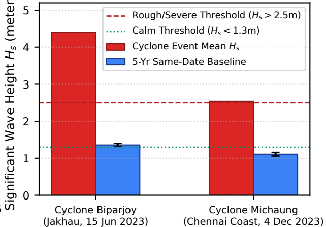
(b) Sea-State vs. Climatology & Fixed Thresholds
