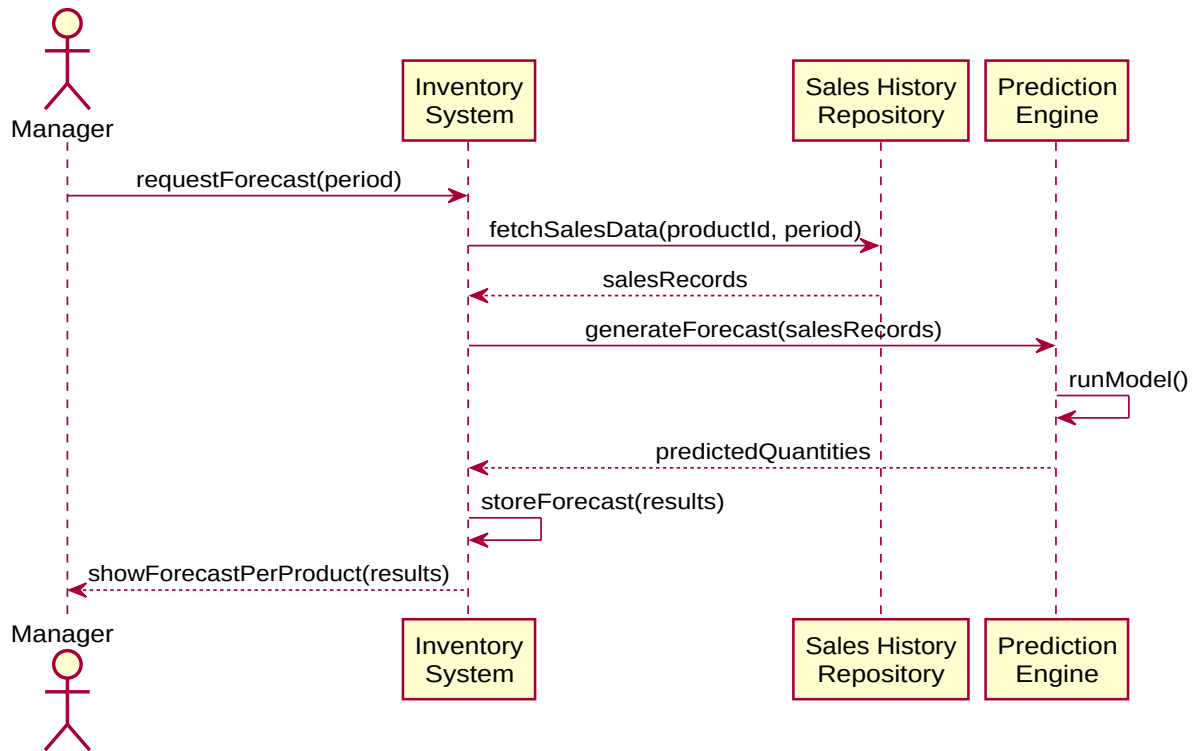
Figure 5.2: Sequence diagram: demand prediction generation
