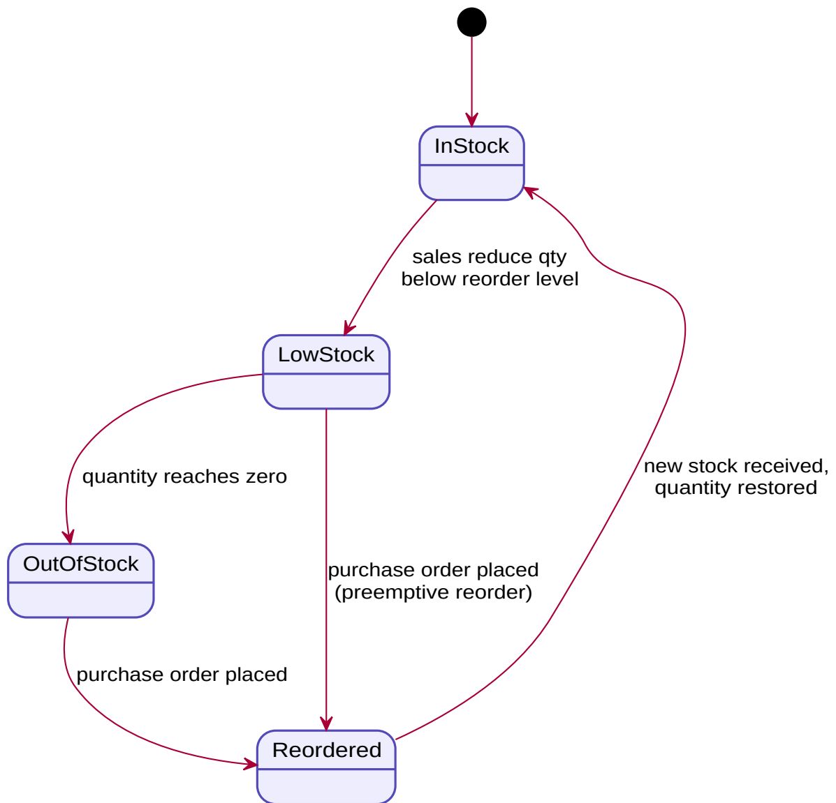
Figure 5.5: State transition diagram: inventory item stock status
