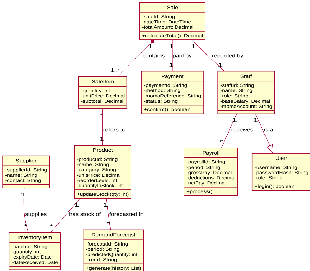
Figure 4.1: Class diagram for SmartStock
