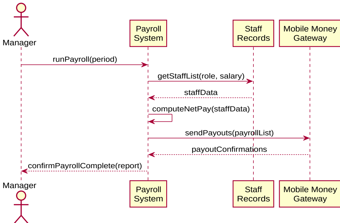
Figure 5.3: Sequence diagram: staff payroll processing
