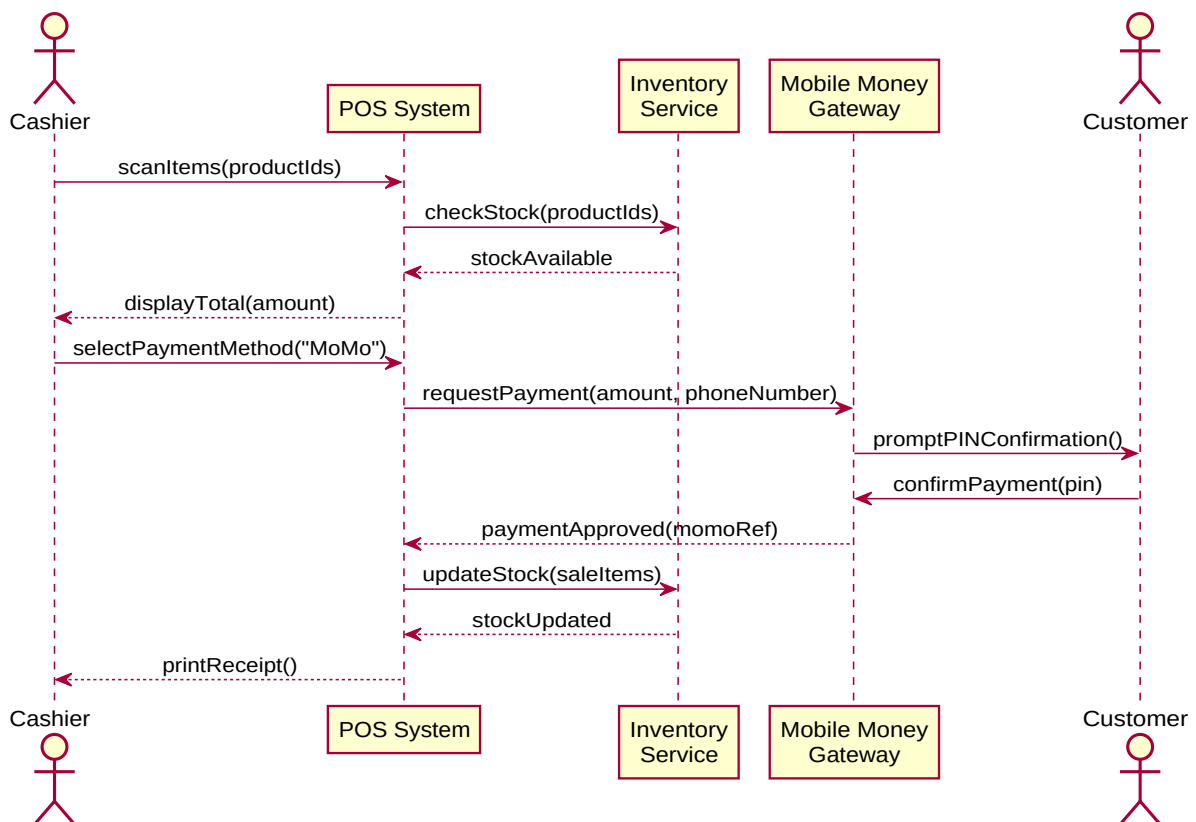
Figure 5.1: Sequence diagram: sale with mobile money payment
