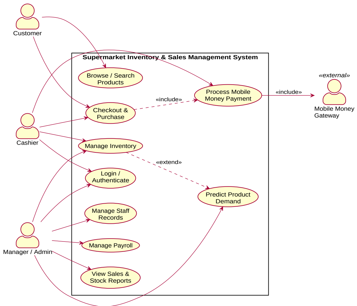
Figure 3.1: Use case diagram for SmartStock
