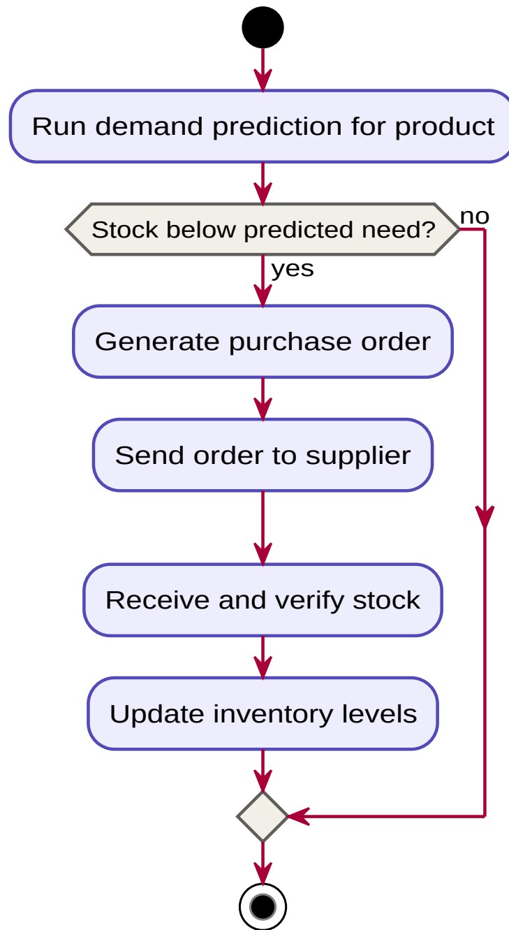
Figure 5.4: Activity diagram: stock replenishment based on prediction
