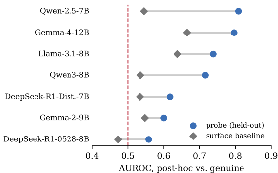
Figure 6: Instructed construction across 7 models: probe held-out AUROC (circles) vs. the surface-feature black-box baseline (diamonds).
