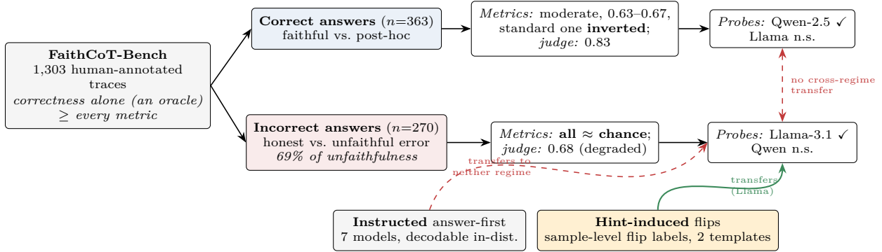
Figure 1: Overview. Stratifying FaithCoT-Bench by correctness splits detection into two regimes, behaviorally and internally; of the constructed testbeds, only hint-induced flip probes transfer to the annotations, onto the metric-blind regime.
