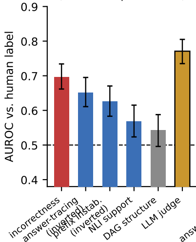
Complete-feature subset (n=633; 2 open models)
