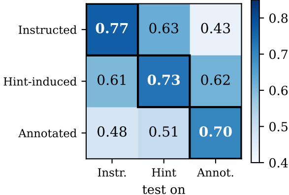
Probe transfer, layer-mean AUROC (Llama)
