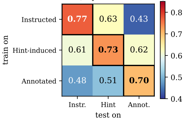
Probe transfer, layer-mean AUROC (Llama)
