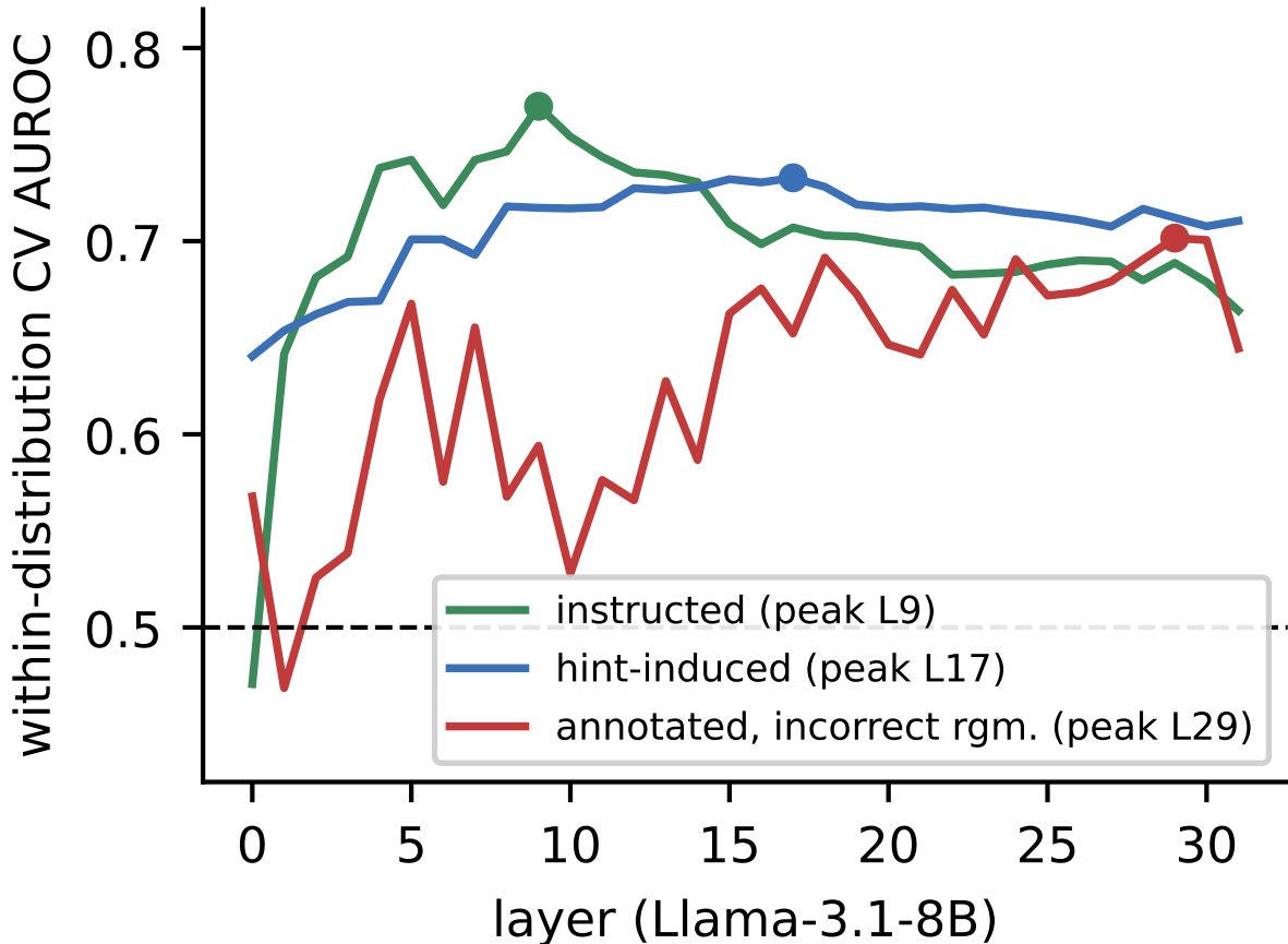
Figure 5: Per-layer probe AUROC for the three constructions (Llama-3.1-8B; descriptive). Instructed peaks early (L9), hint-induced mid (L17), annotated incorrect-regime late (L29); peak locations may be unstable under resampling.
