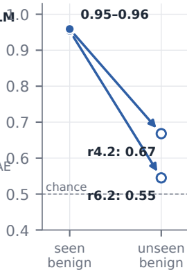
ROC collapse
