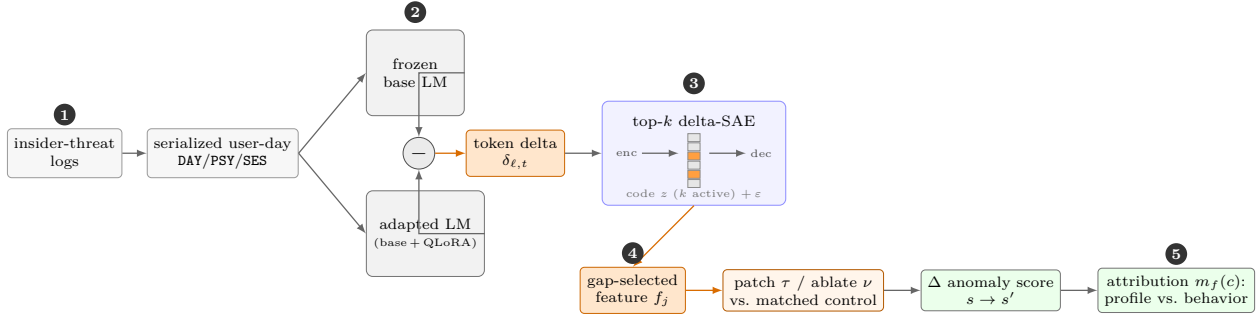
Figure 2: The delta-SAE audit, drawn as architecture. (1) A user-day is serialized into structured DAY/PSY/SES text. (2) The same input runs through the frozen base model and its benign-only QLoRA-adapted copy; at layer \ell we take the per-token residual-stream difference \delta_{\ell,t} = h_{\ell,t}^{\text{ada}} - h_{\ell,t}^{\text{base}} (the adapter is left abstract—the delta is the object of study). (3) \delta feeds a top- k sparse autoencoder (encoder \rightarrow sparse code z with only k units active, shown as the lit cells \rightarrow decoder, plus reconstruction error), whose decoder columns form the feature dictionary. (4) A gap-selected feature f_j is causally patched ( \tau ) or ablated ( \nu ) against a matched active control, and the effect on the adapted anomaly score s \rightarrow s' is measured. (5) Token attribution m_f(c) labels the feature’s content as profile- or behavior-bound. A mechanistic claim requires both causal relevance (Step 4) and content (Step 5); formal definitions are in Section 4.1.
