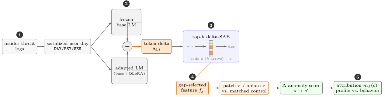
Figure 2: The delta-SAE audit, drawn as architecture. (1) A user-day is serialized into structured DAY/PSY/SES text. (2) The same input runs through the frozen base model and its benign-only QLoRA-adapted copy; at layer \ell we take the per-token residual-stream difference \delta_{\ell,t} = h_{\ell,t}^{\text{ada}} - h_{\ell,t}^{\text{base}} (the adapter is left abstract—the delta is the object of study). (3) \delta feeds a top- k sparse autoencoder (encoder \rightarrow sparse code z with only k units active, shown as the lit cells \rightarrow decoder, plus reconstruction error), whose decoder columns form the feature dictionary. (4) A gap-selected feature f_j is causally patched ( \tau ) or ablated ( \nu ) against a matched active control, and the effect on the adapted anomaly score s \rightarrow s' is measured. (5) Token attribution m_f(c) labels the feature’s content as profile- or behavior-bound. A mechanistic claim requires both causal relevance (Step 4) and content (Step 5); formal definitions are in Section 4.1.
