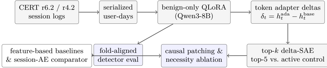
Figure 1: Overview. Session logs are serialized into structured user-day text and used to adapt Qwen3-8B on benign users only. Token-level adapter deltas feed sparse top- k autoencoders whose feature sets are evaluated by causal patching and necessity ablation against active controls with same-user donors excluded. Detector comparisons against the feature-based one-class baselines use a shared fold-aligned protocol.
