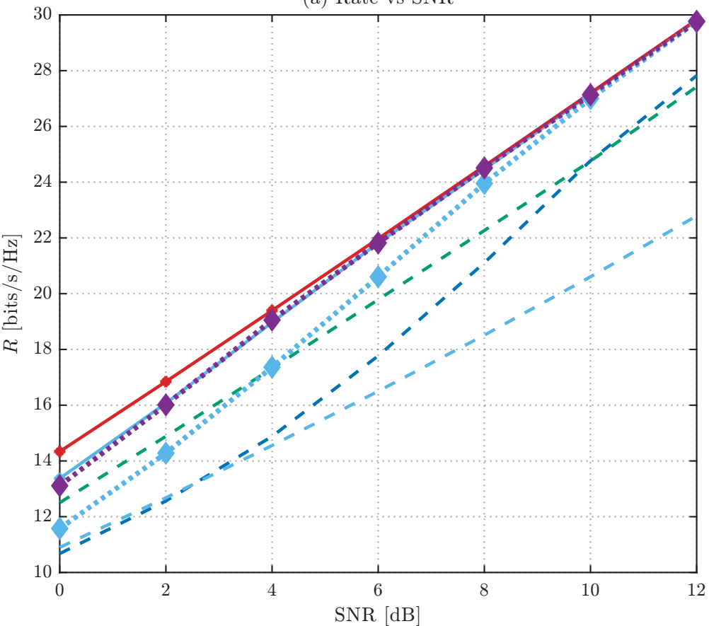
(a) Rate vs SNR
