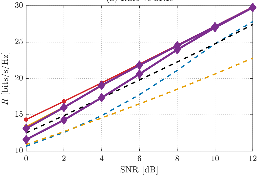
(a) Rate vs SNR
