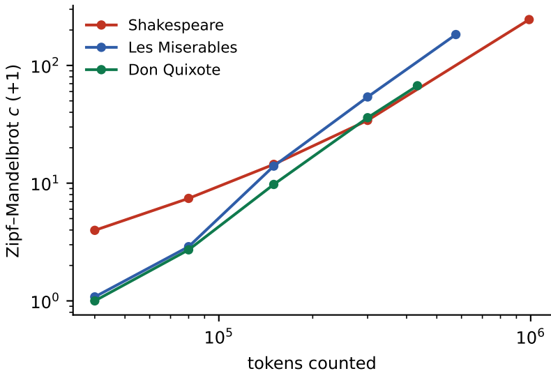
Mandelbrot's c collapses with sampling depth
