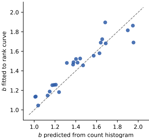
Histogram predicts the exponent ( r = 0.941 )
