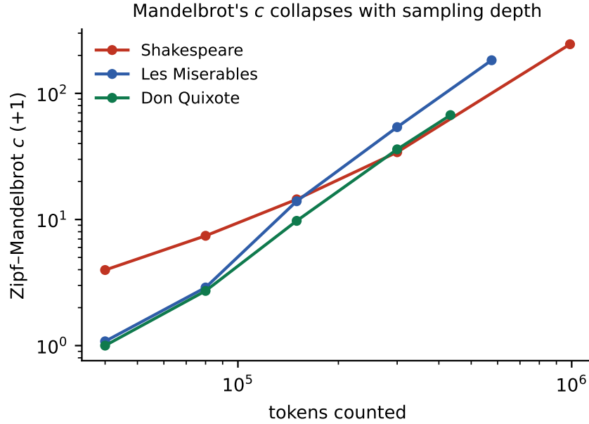
Figure 3: Subsampling collapses the fitted shift c along smooth trajectories.
