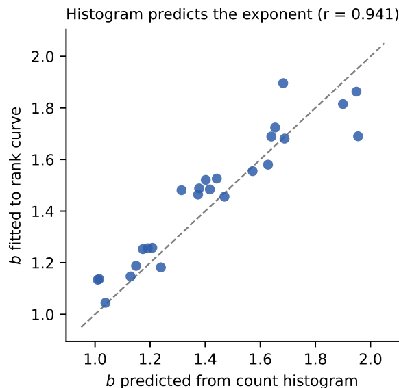
Figure 4: The exponent predicted from the count histogram alone versus the exponent fitted to the rank curve (25 corpora).
