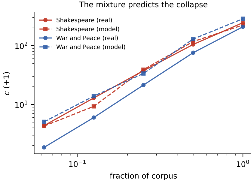
Figure 5: Downward c(T) trajectories: binomially thinned data (circles) versus the mixture fitted at full depth (squares).
