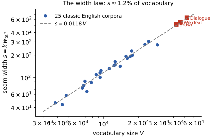
Figure 2: The width law: seam width s against vocabulary V for 25 classic corpora (circles) and three modern registers (squares), with s = 0.0118 V .
