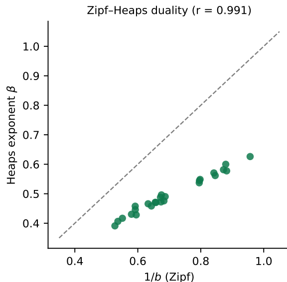
Figure 6: Heaps’ exponent against 1/b : the measured Zipf–Heaps duality ( r = 0.991 ).
