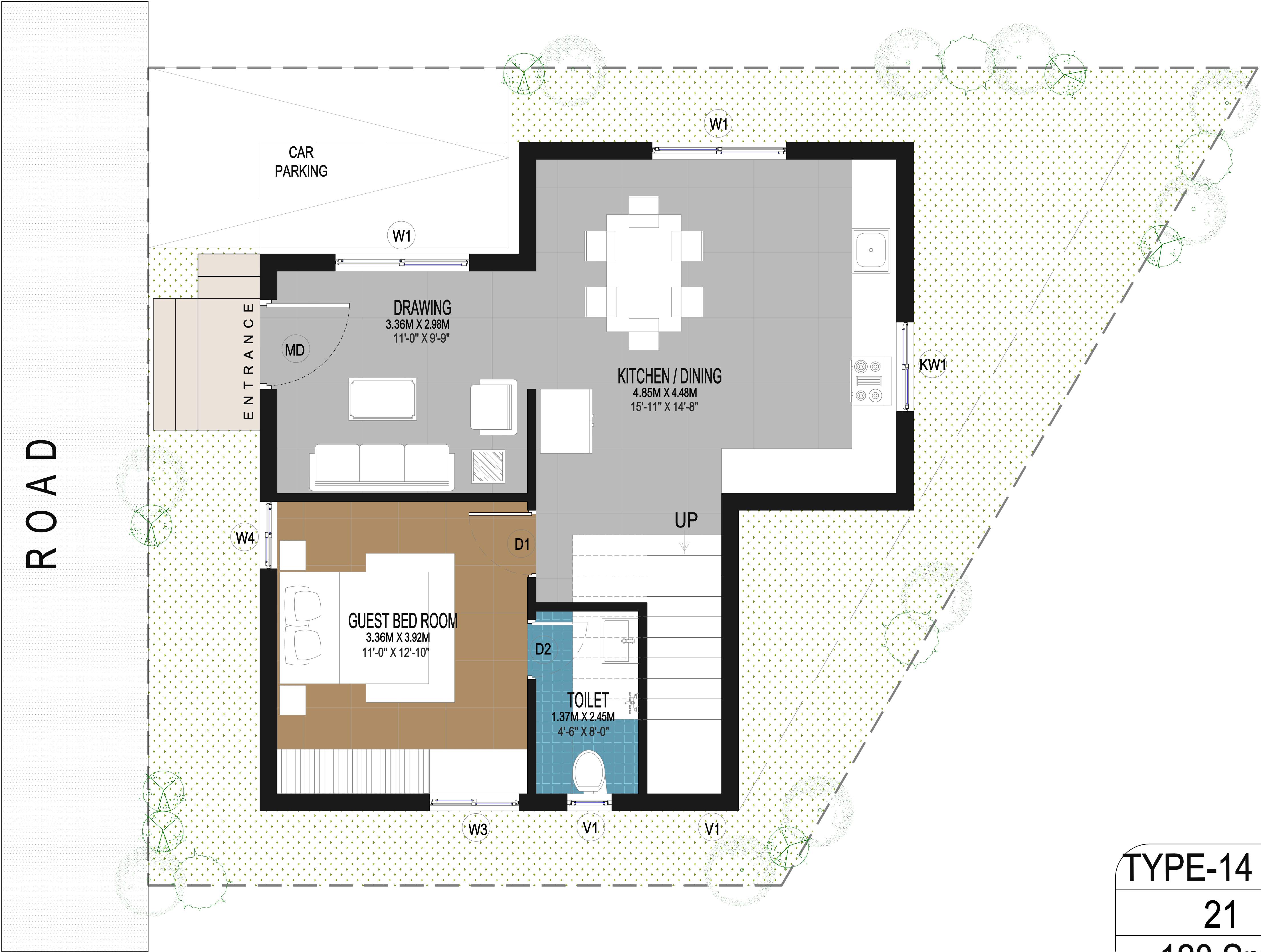
GF - GROUND FLOOR PLAN
