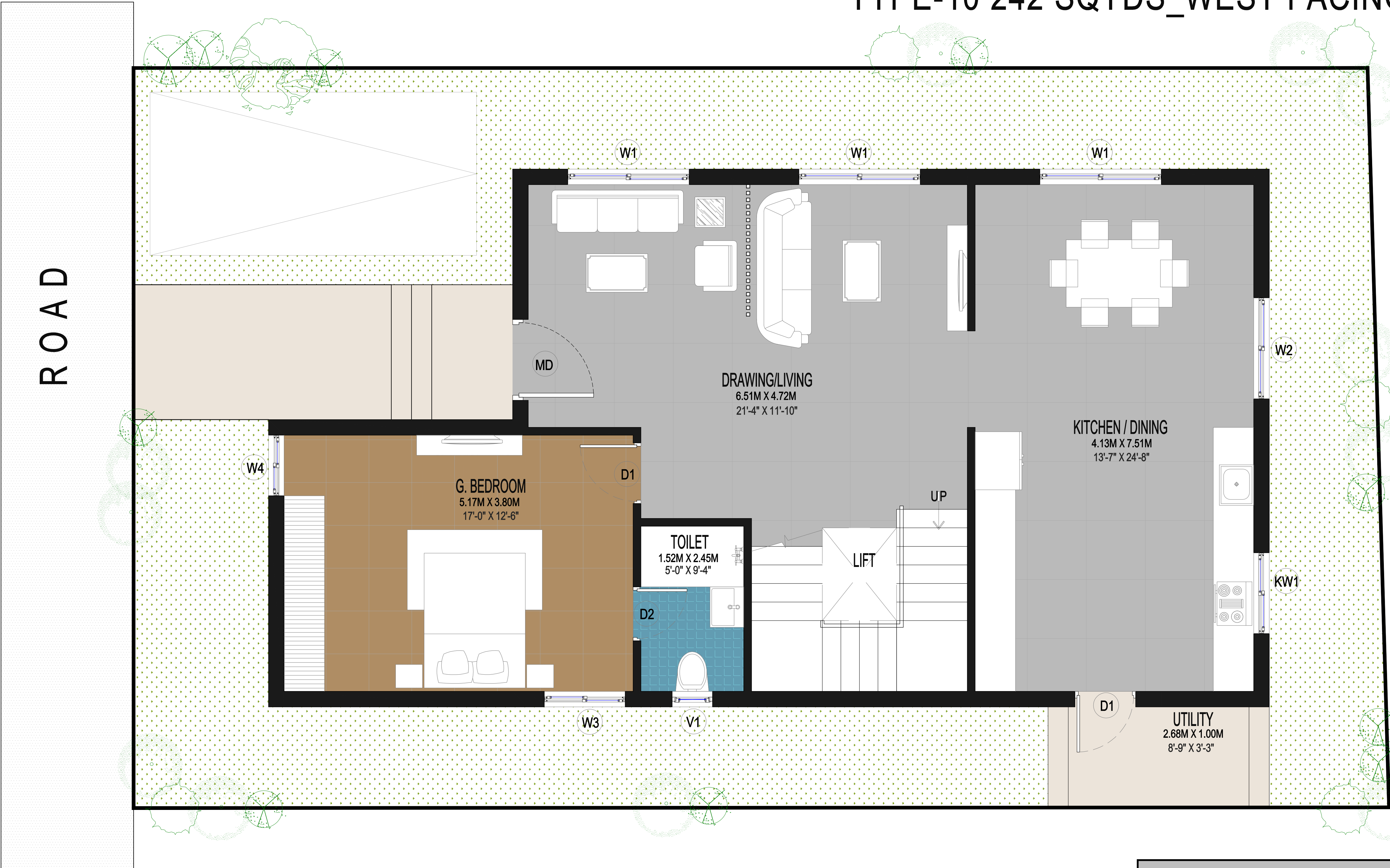
GF GROUND FLOOR PLAN
