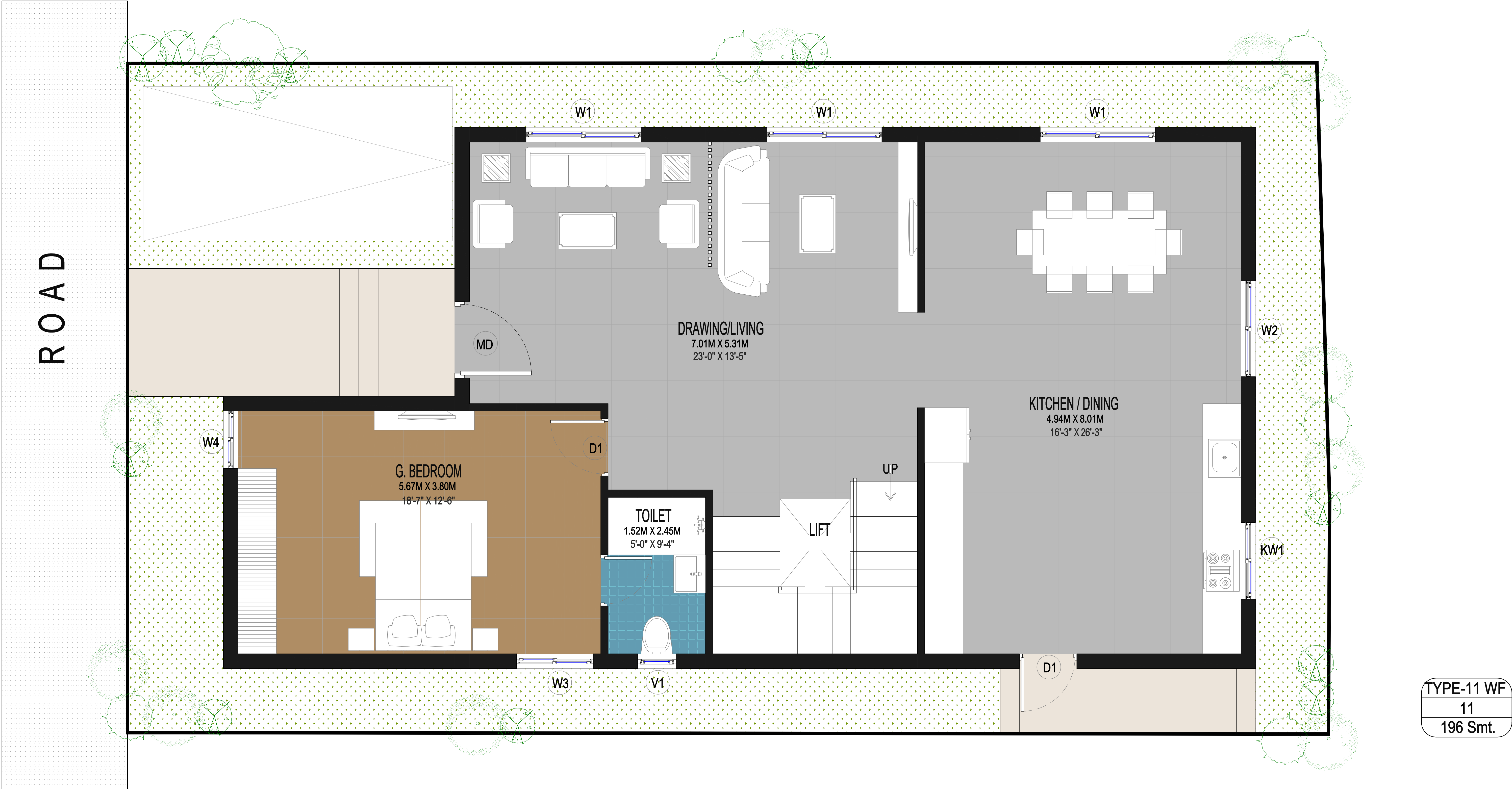
GF - GROUND FLOOR PLAN
