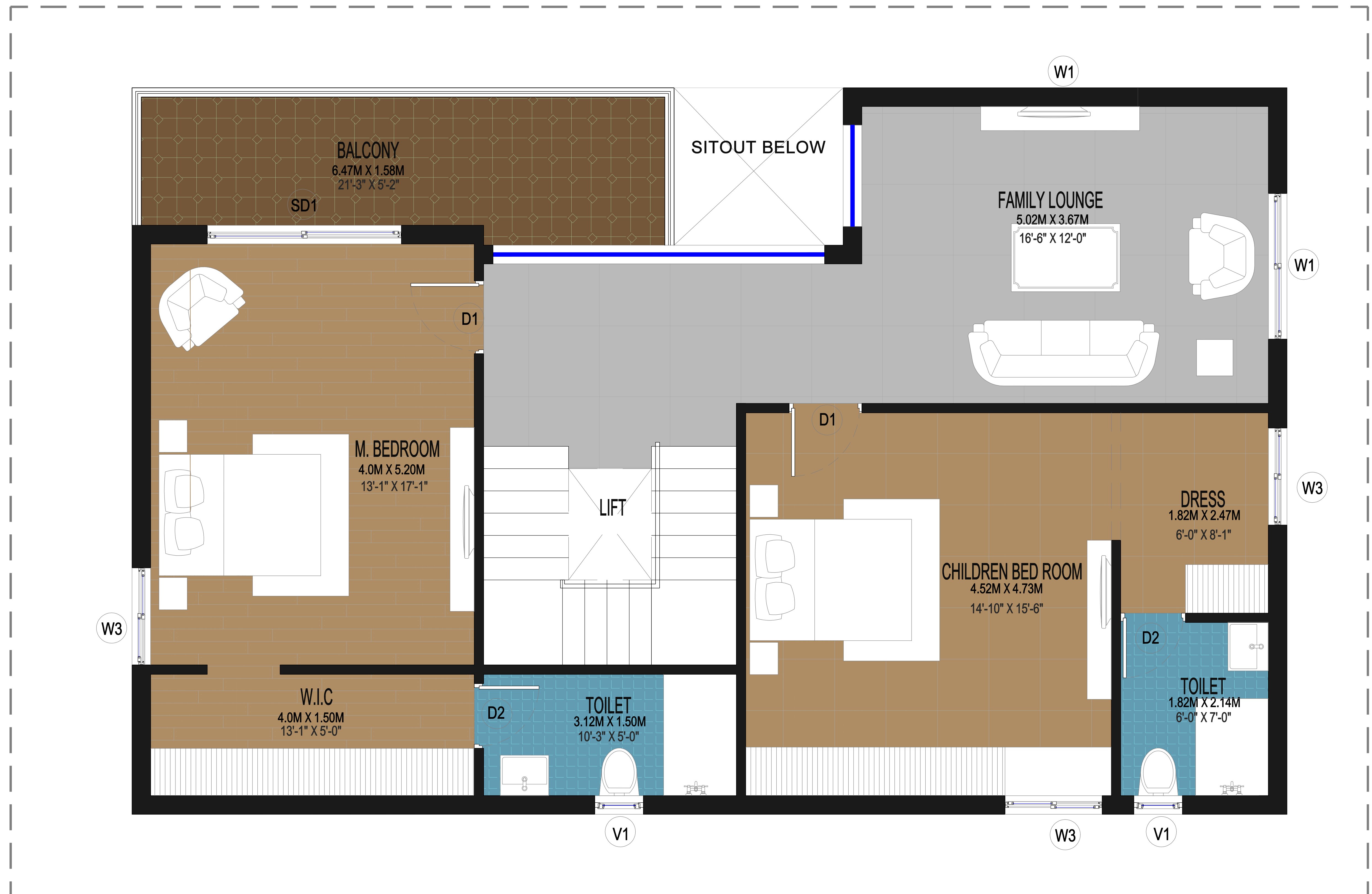
FF - FIRST FLOOR PLAN
