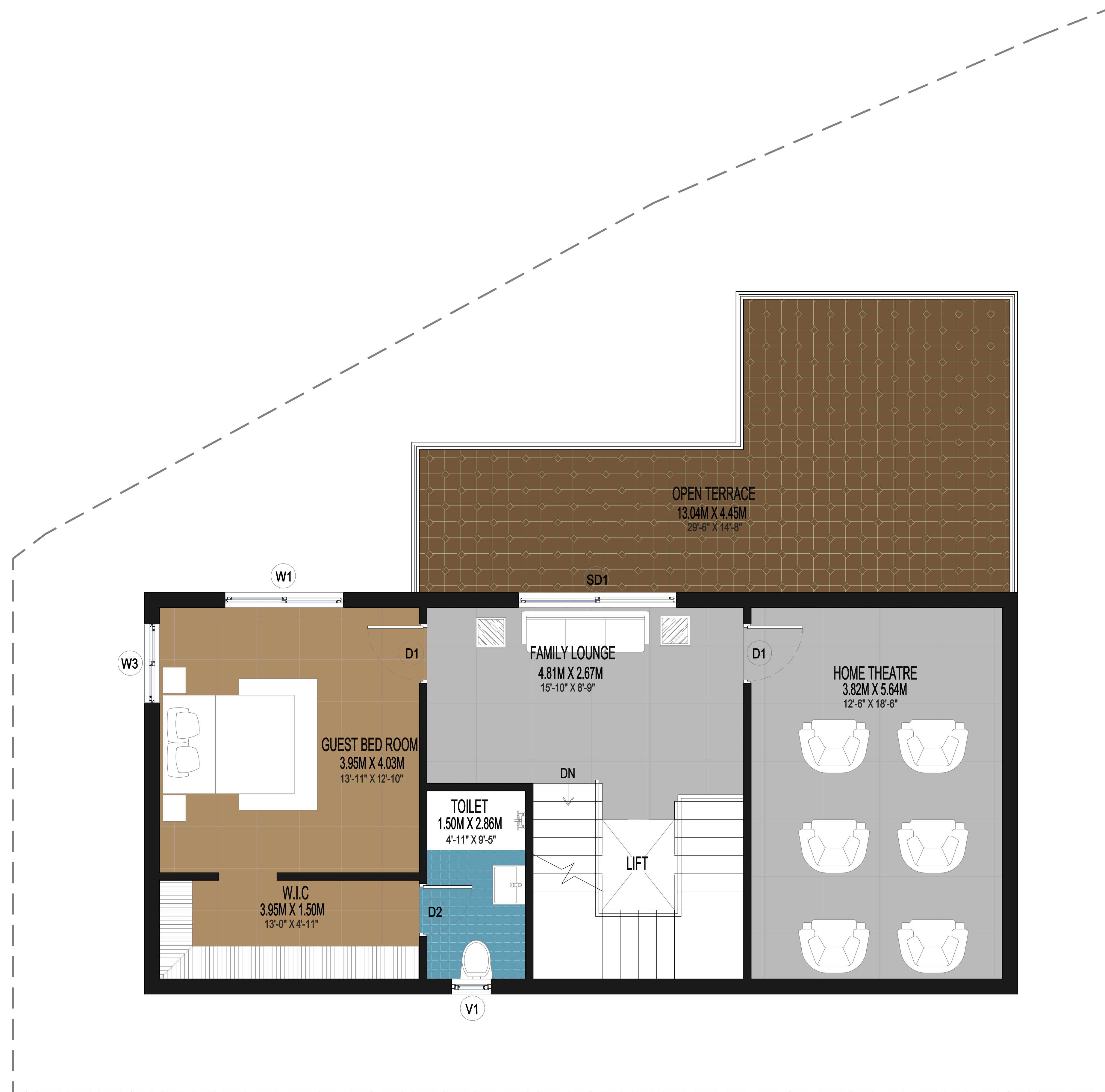
SF - SECOND FLOOR PLAN
