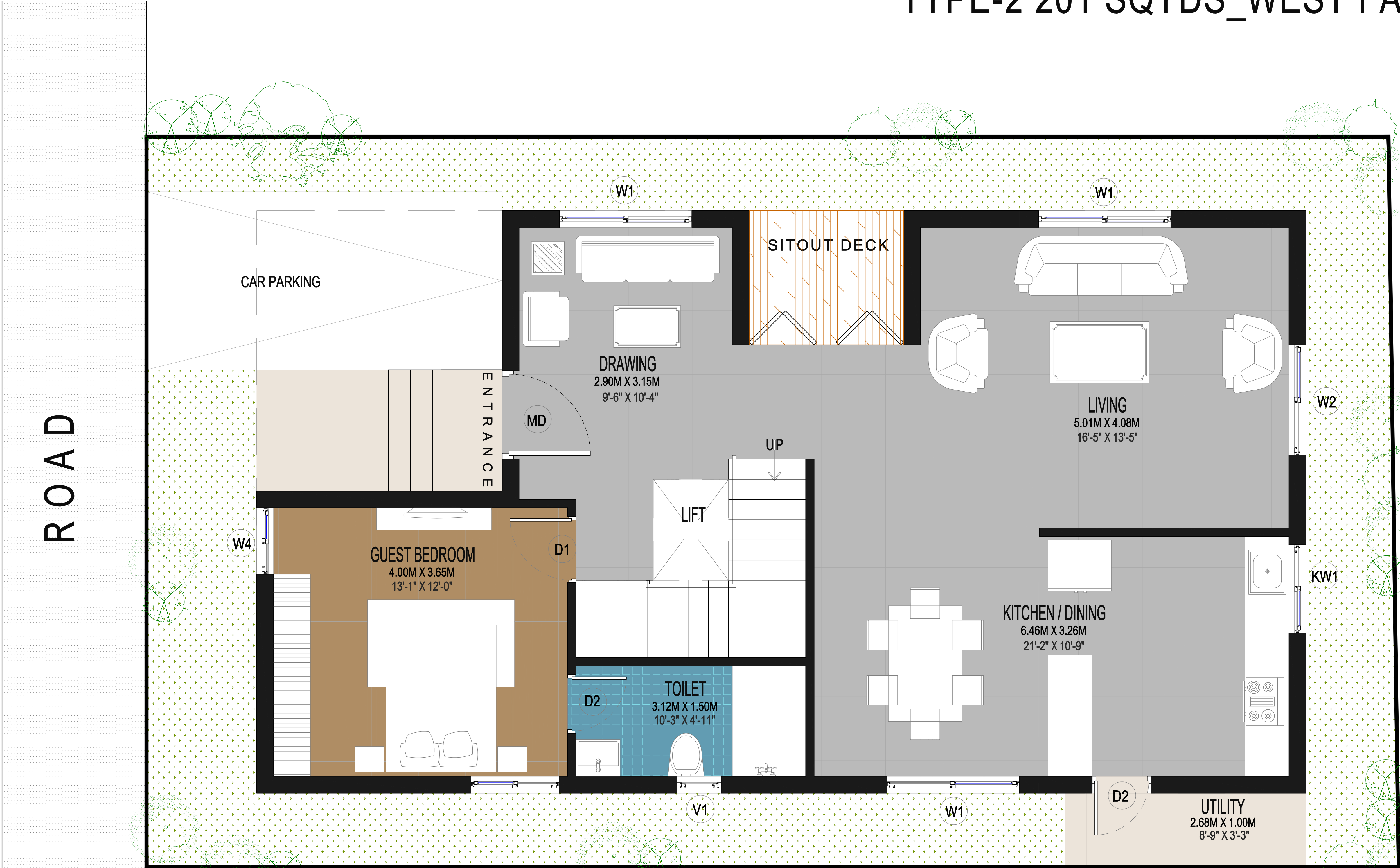
GF - GROUND FLOOR PLAN
