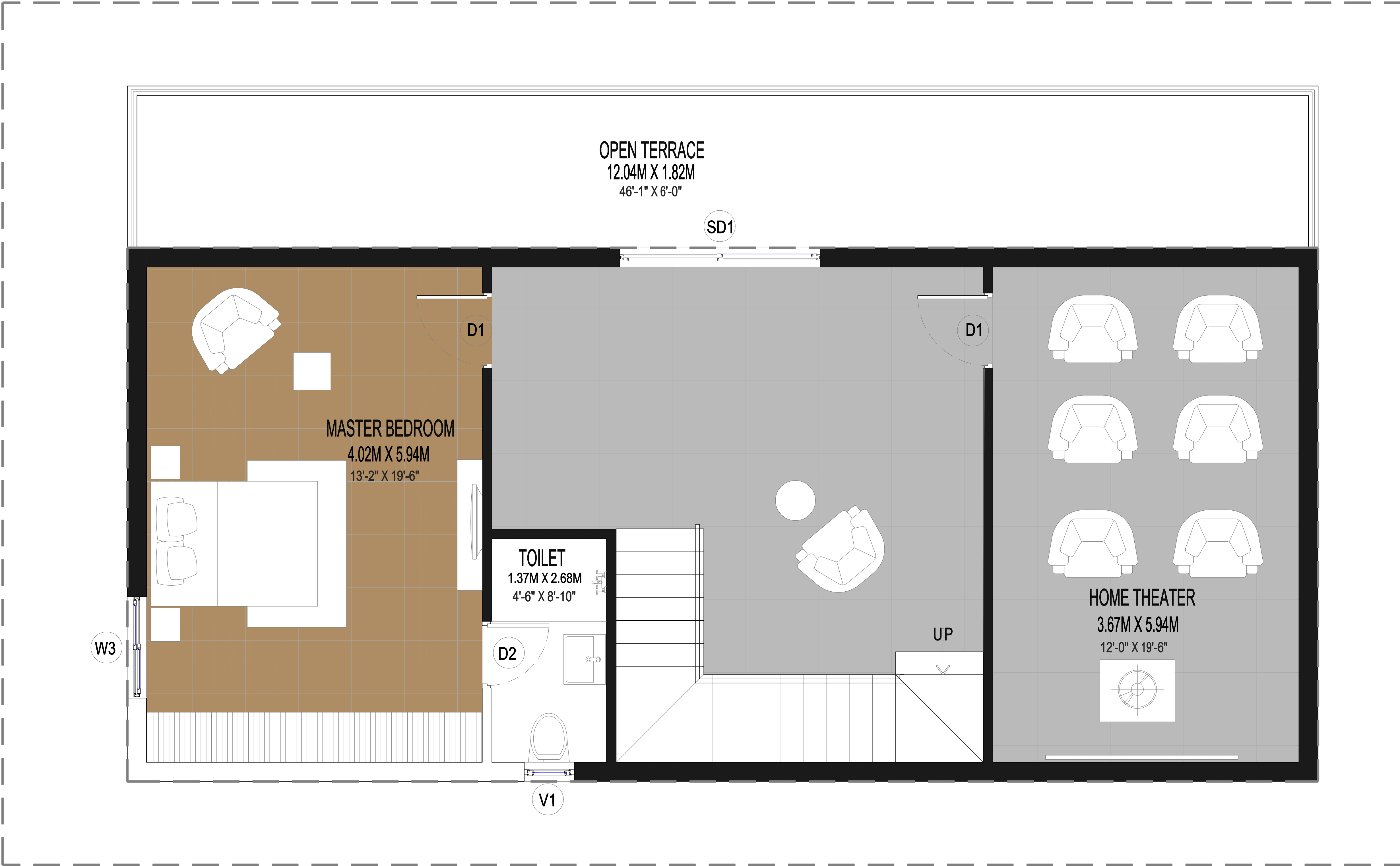
SF - SECOND FLOOR PLAN
