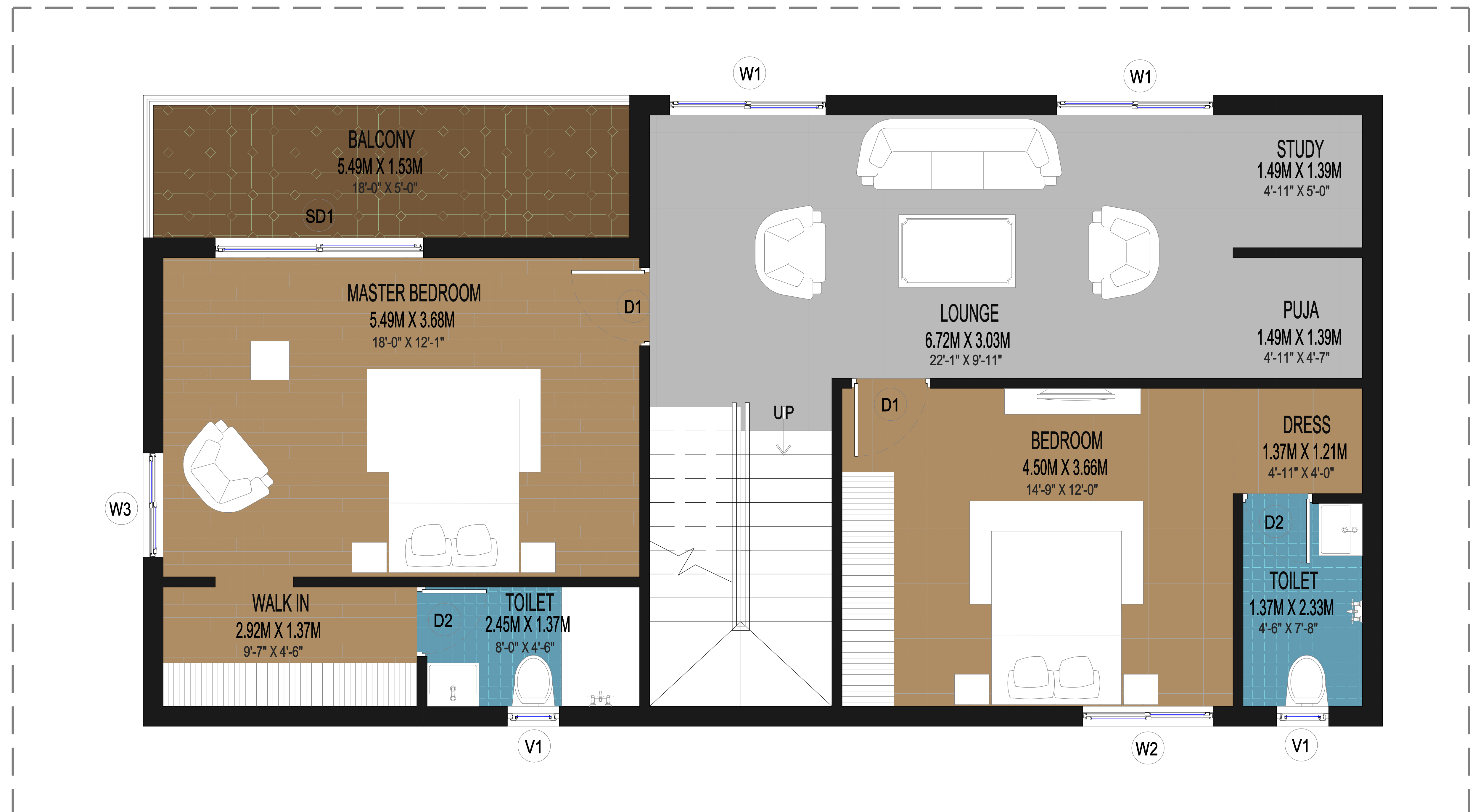
FF - FIRST FLOOR PLAN
