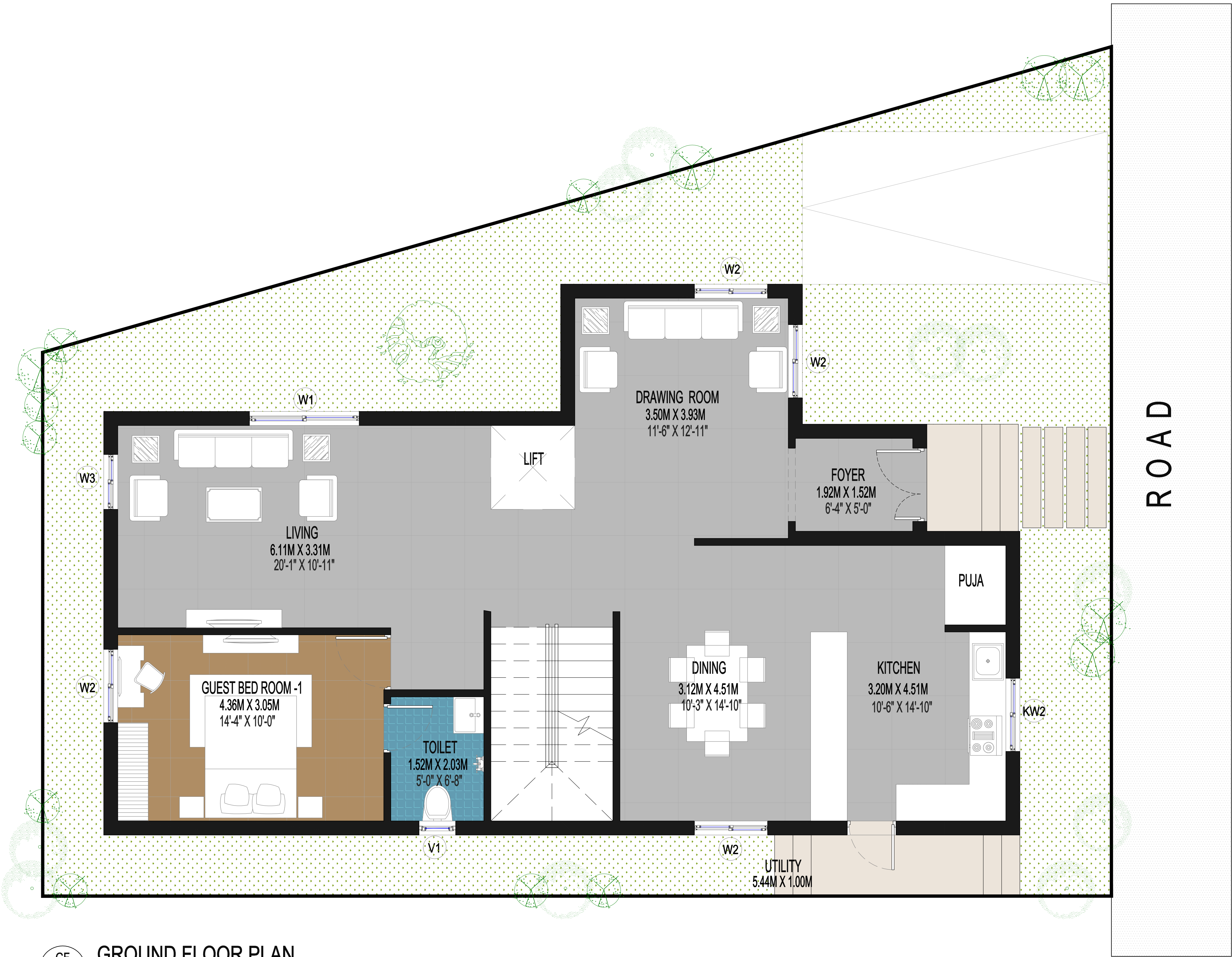
GF GROUND FLOOR PLAN
