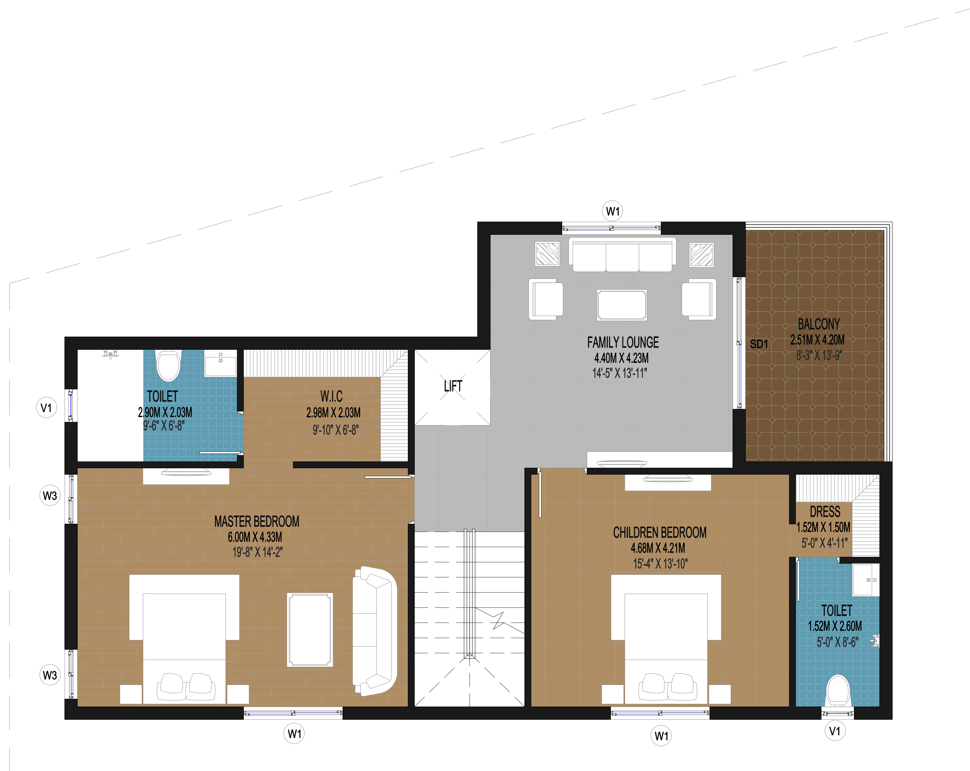
FF FIRST FLOOR PLAN
