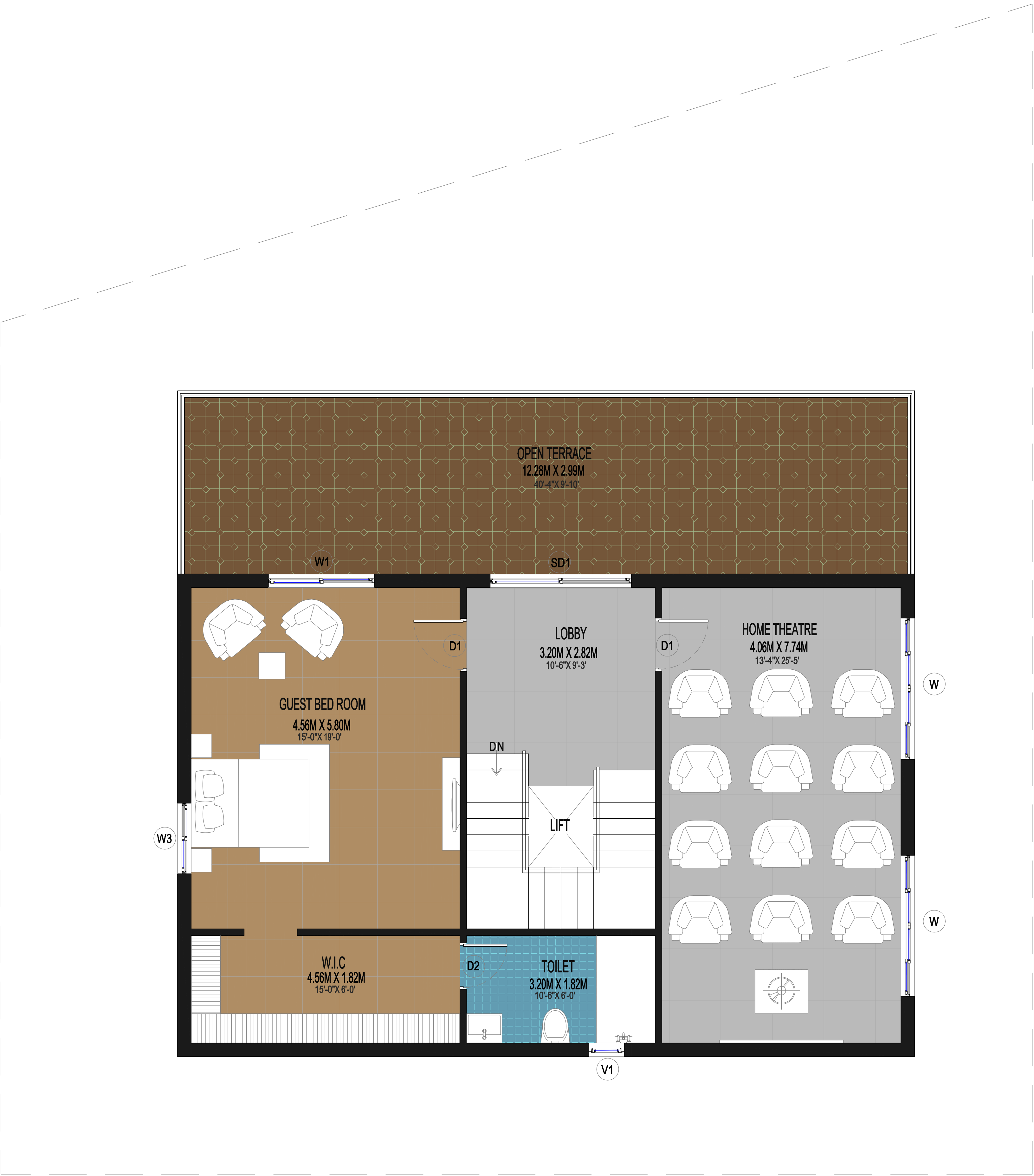
SF - SECOND FLOOR PLAN
