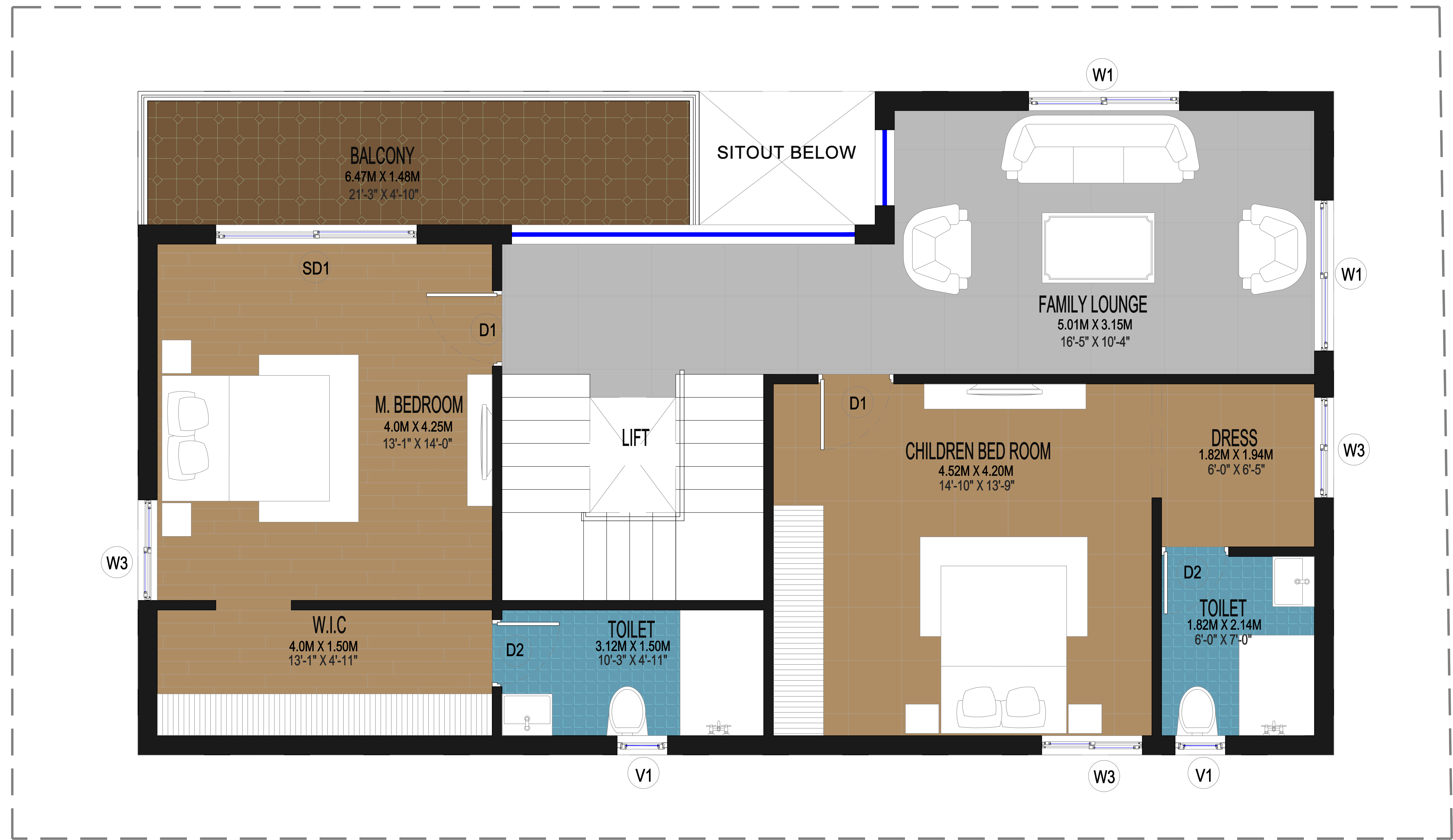
FF - FIRST FLOOR PLAN
