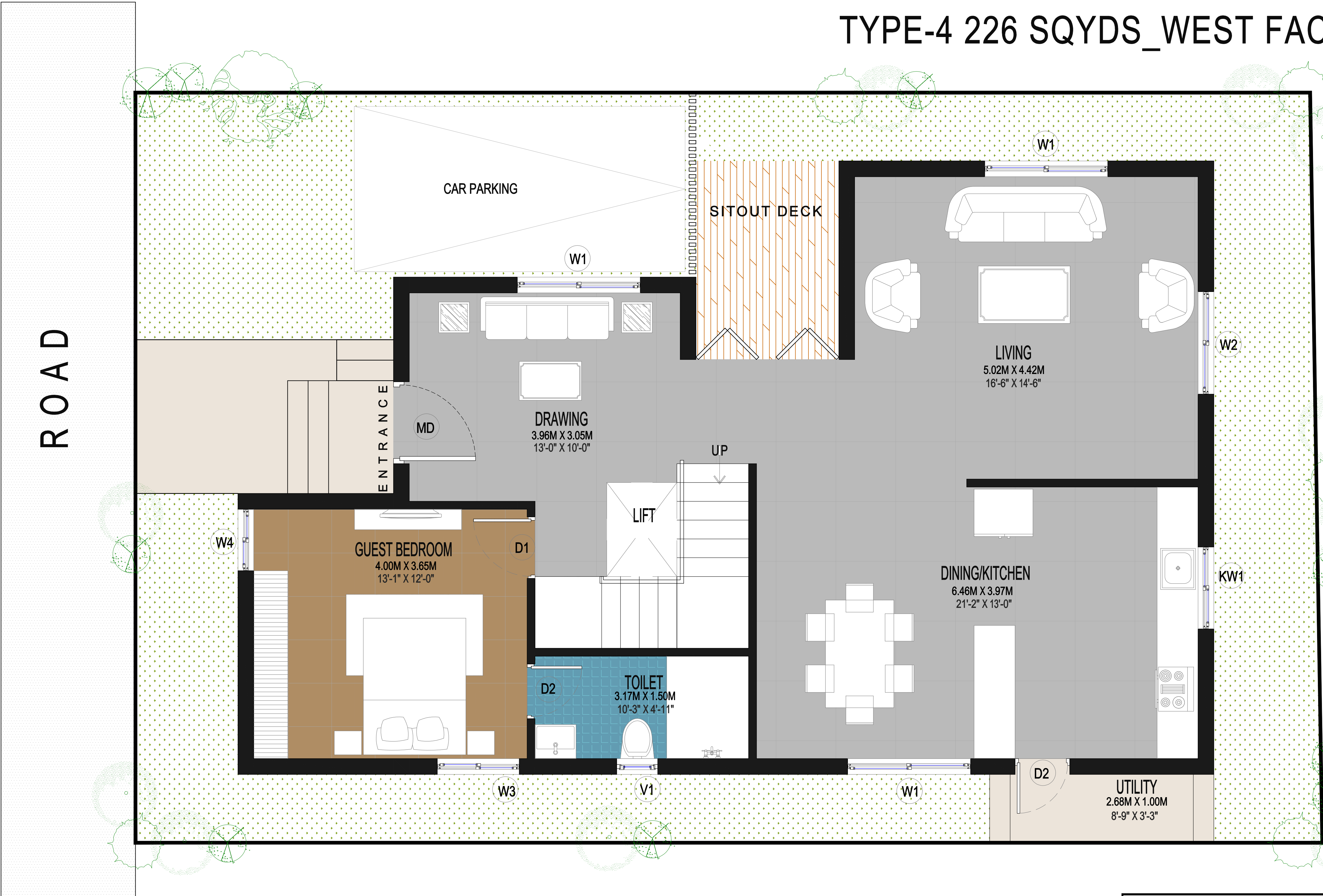
GF - GROUND FLOOR PLAN
