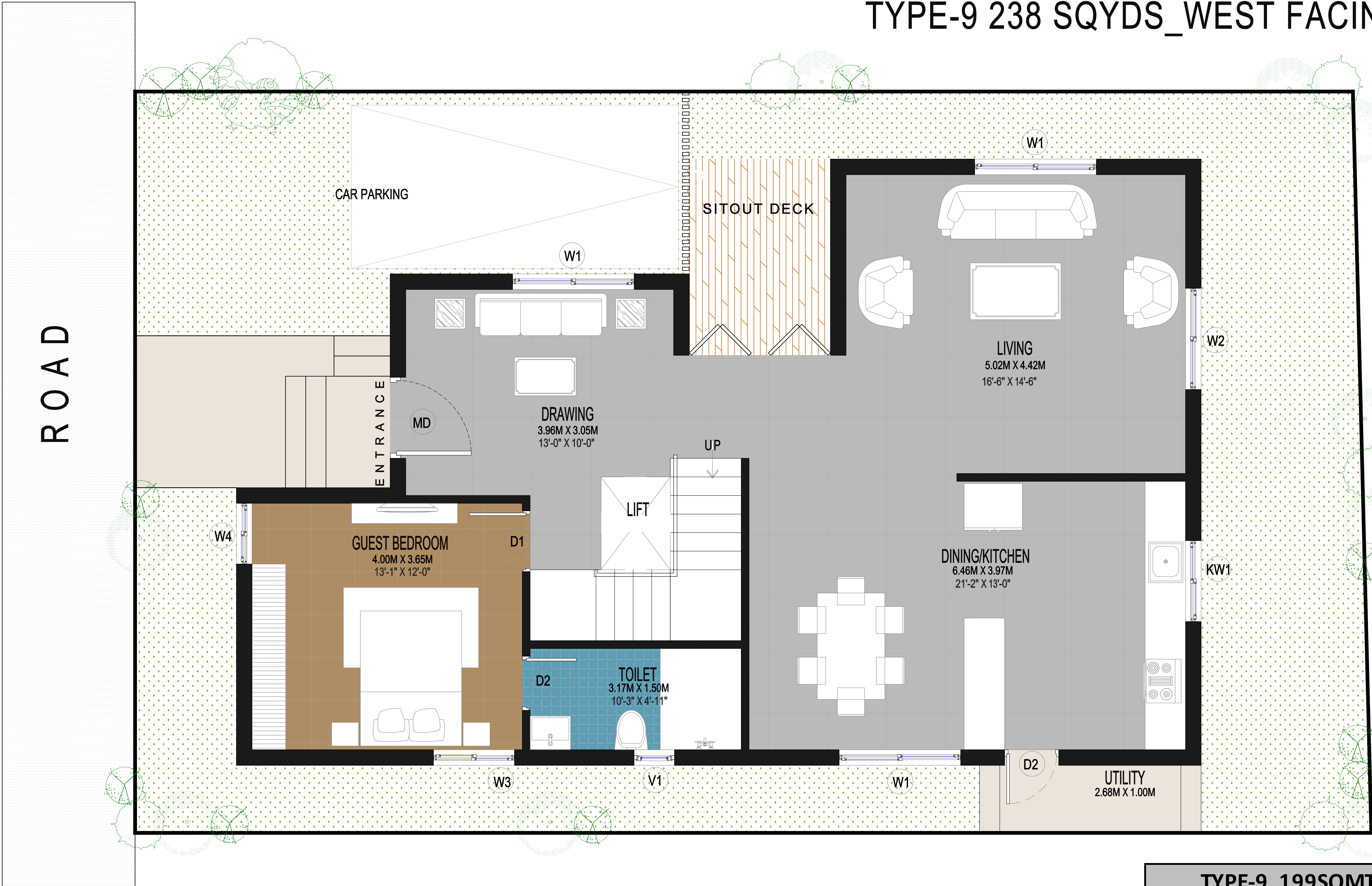
GF GROUND FLOOR PLAN
