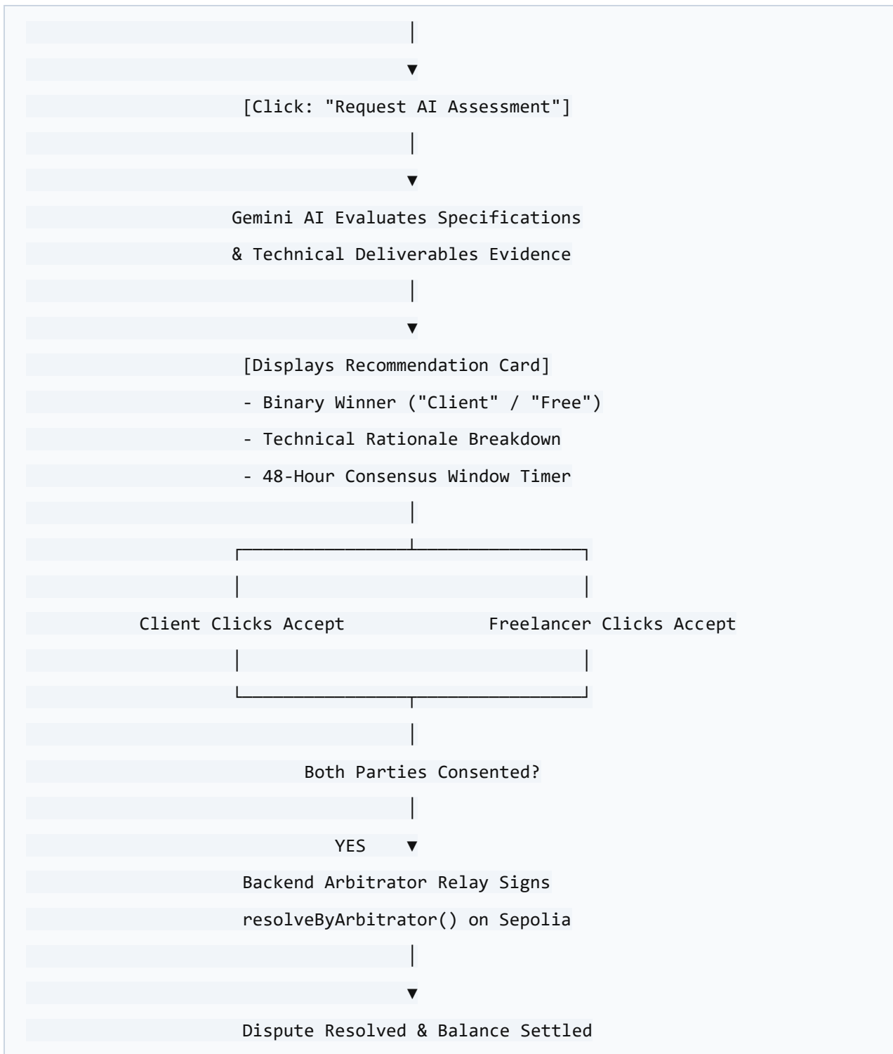
Figure 3.4: AI Dispute Consensus State Transition Diagram
