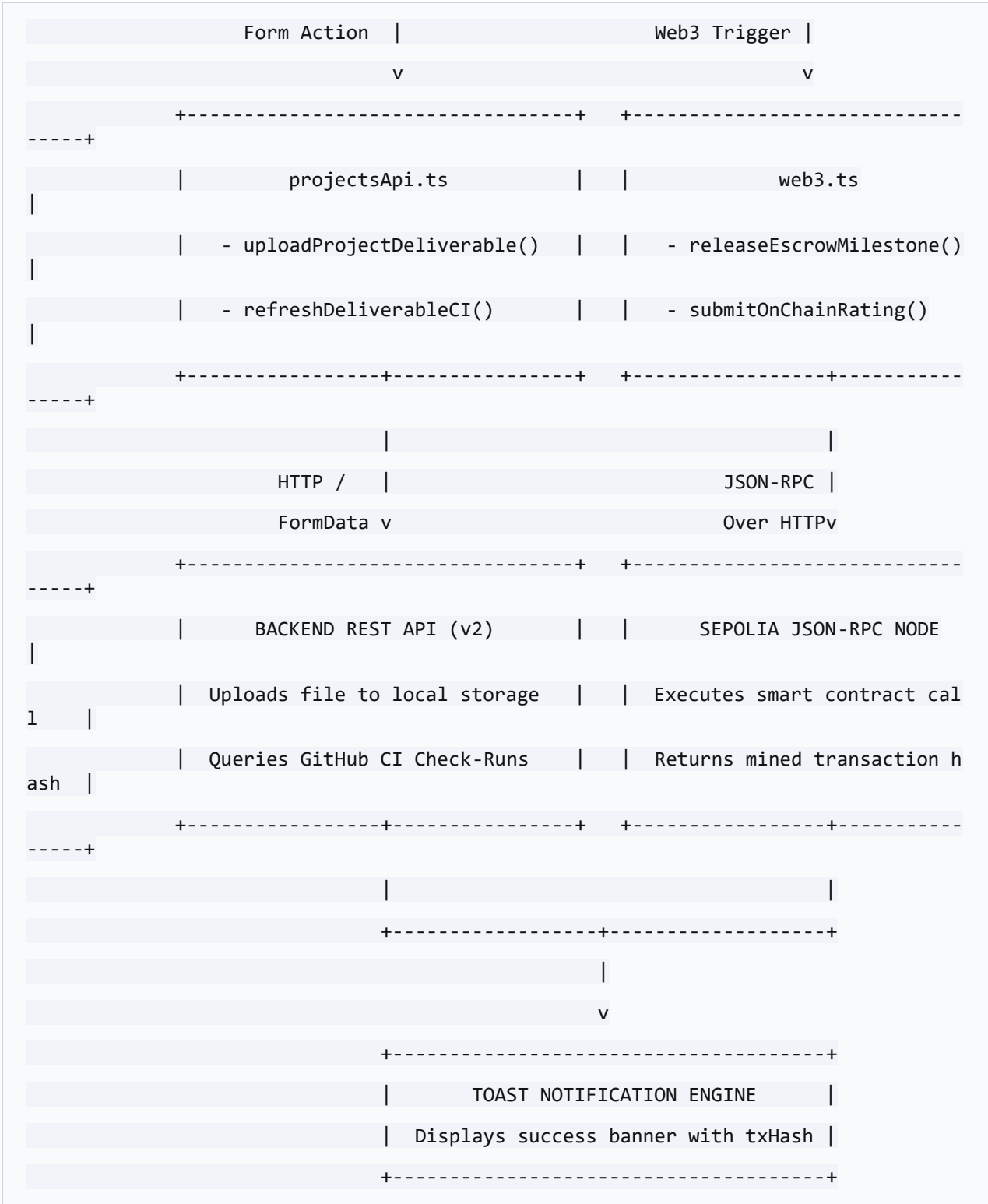
Figure 3.5: Frontend Level 1 Data Flow Diagram
