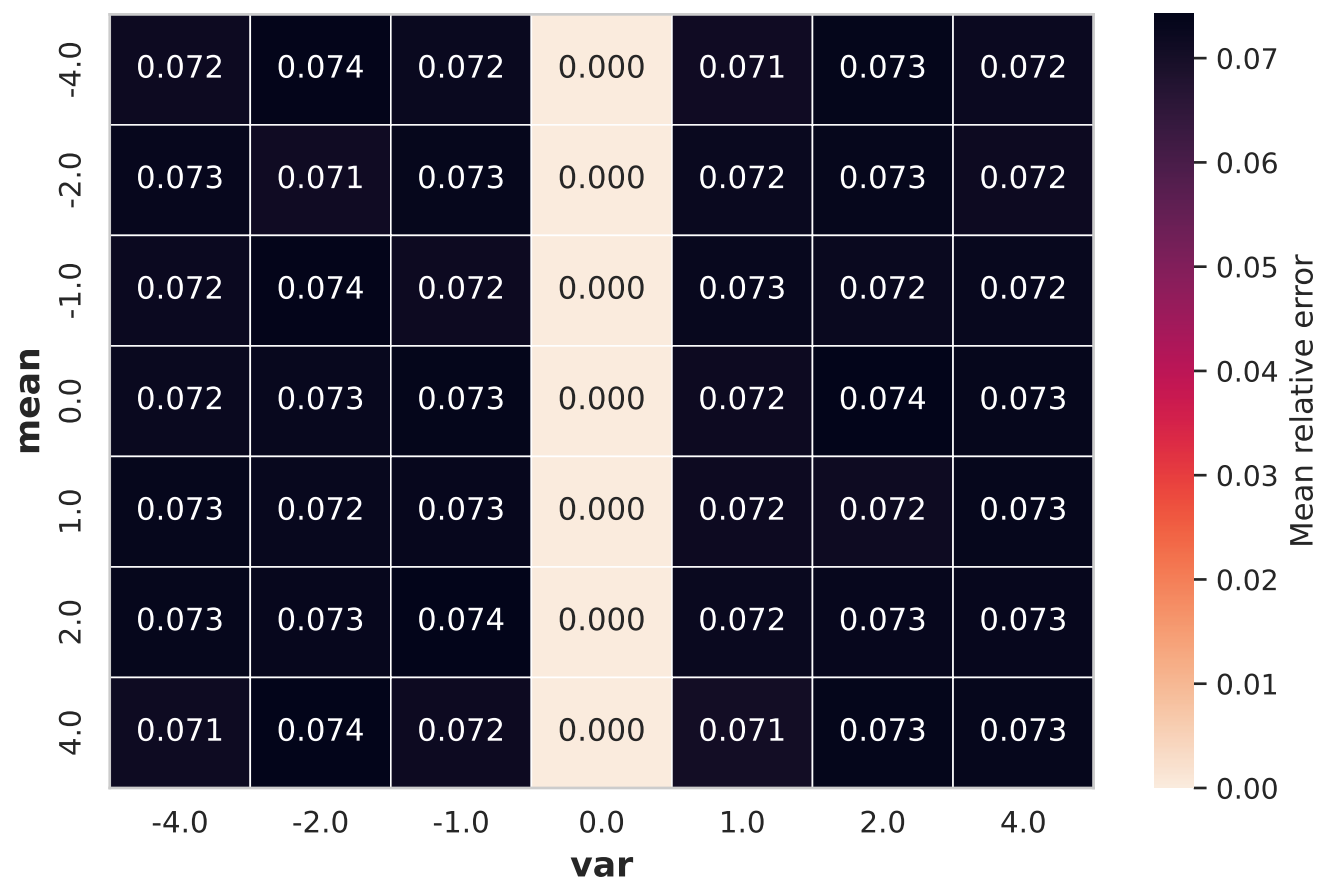
Relative Error: Mean vs Var
