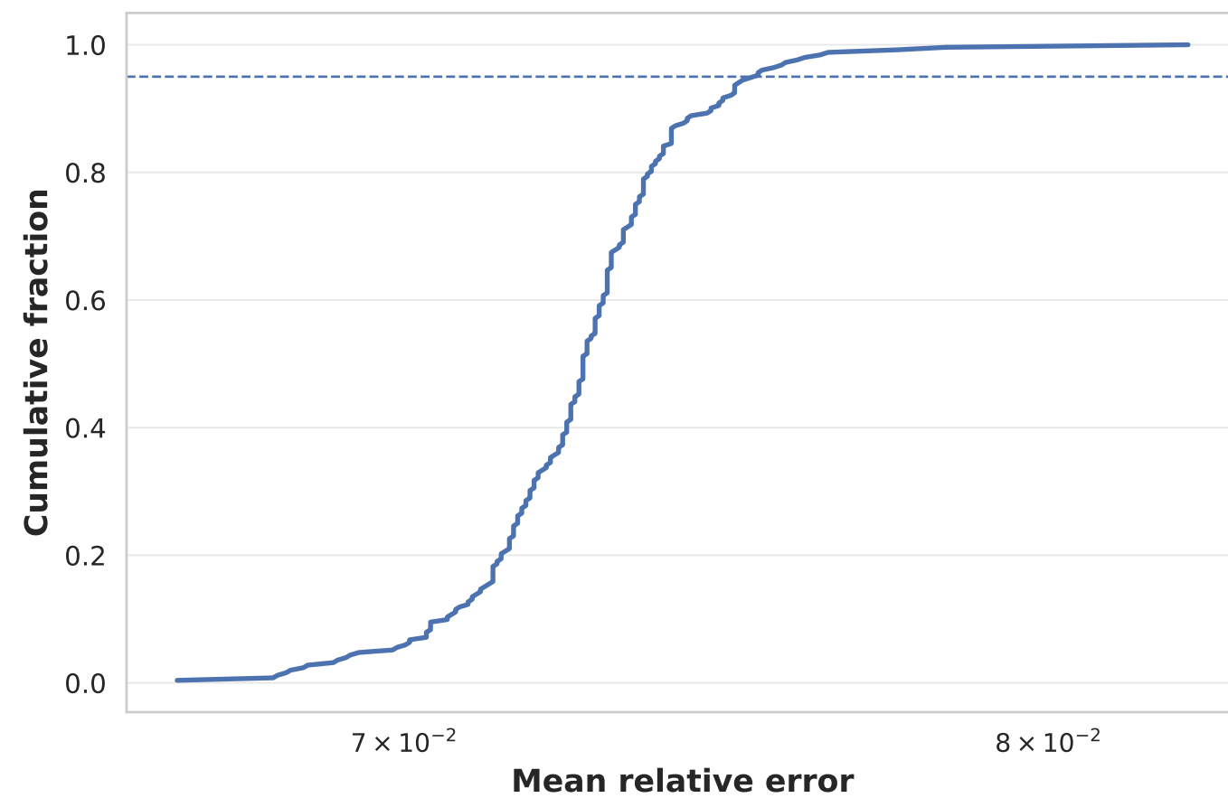
Distribution of Relative Error
