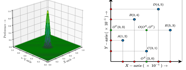
(a) A sample 2-D preference. (b) Preference projections.
