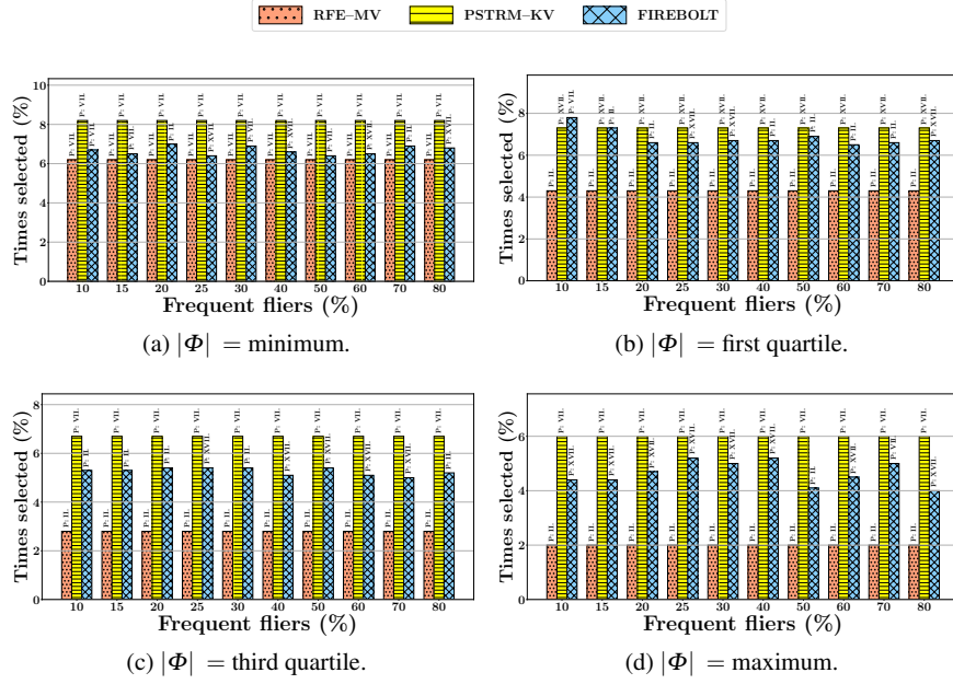
Fig. 3 Percentage of times the most frequently selected fifth project got selected across all simulations of the mechanisms for different percentages of frequent fliers during dishonest voting for different numbers of residents |\Phi| in the variation range.
