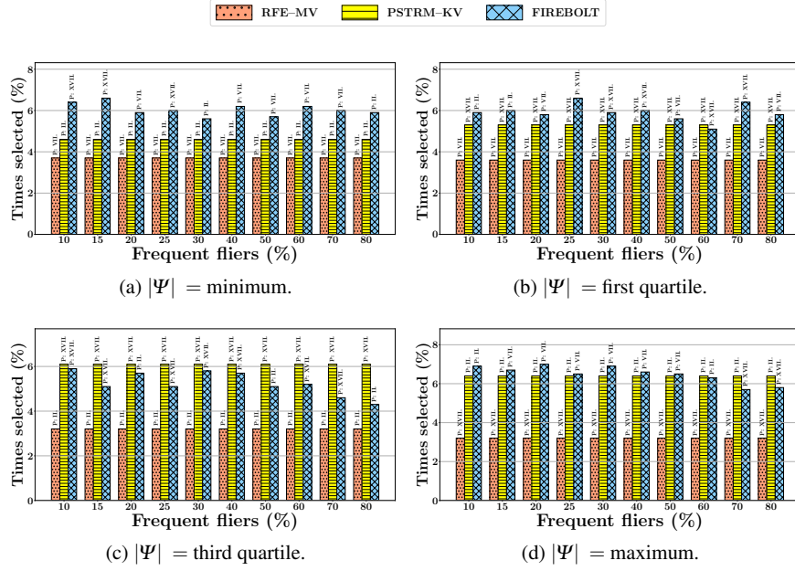
Fig. 2 Percentage of times the most frequently selected fifth project got selected across all simulations of the mechanisms for different percentages of frequent fliers during honest voting for different numbers of ministers |\Psi| in the variation range.
