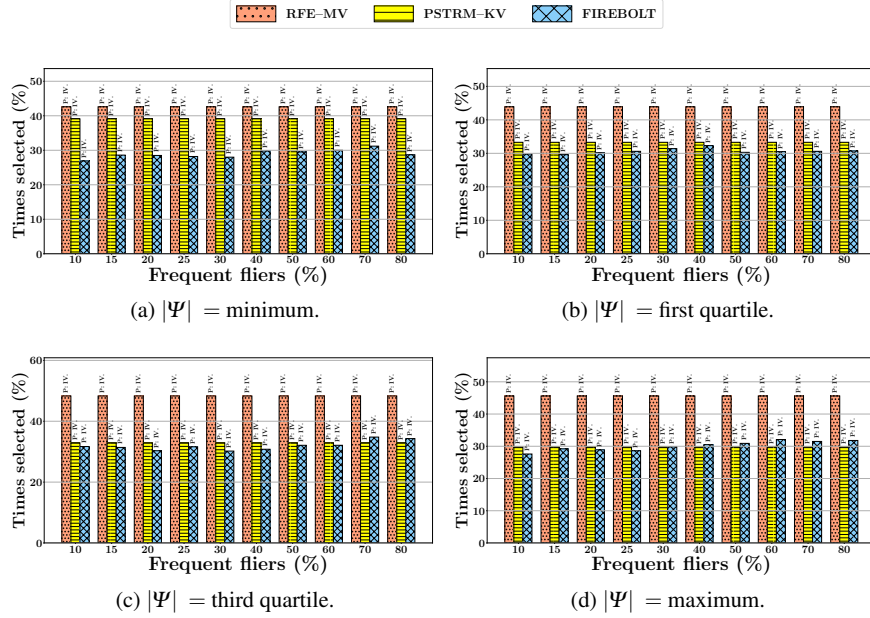
Fig. 1 Percentage of times the most frequently selected first project got selected across all simulations of the mechanisms for different percentages of frequent fliers during honest voting for different numbers of ministers |\Psi| in the variation range.
