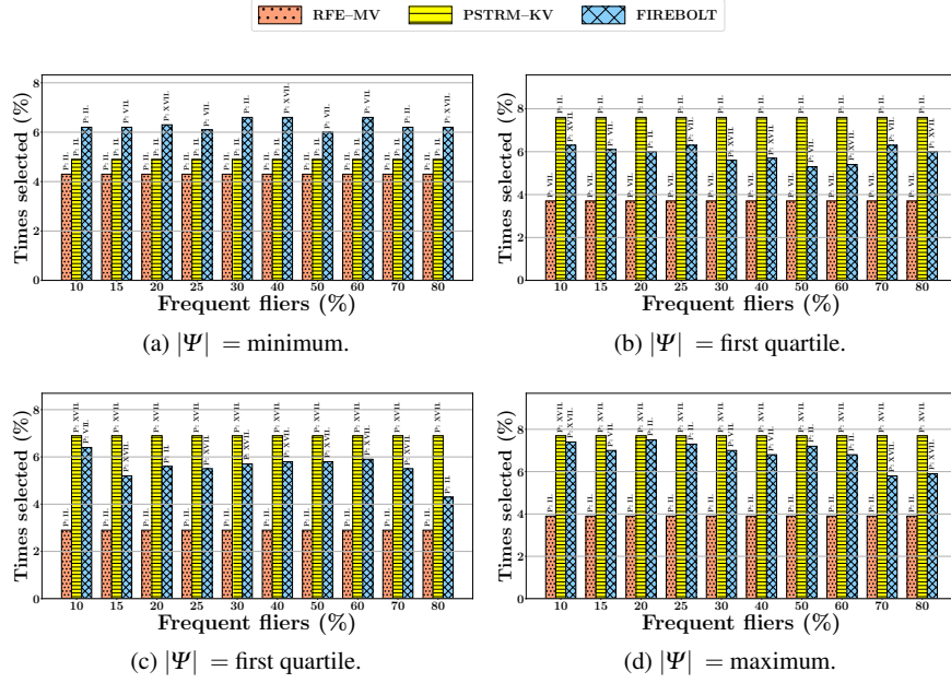
Fig. 4 Percentage of times the most frequently selected fifth project got selected across all simulations of the mechanisms for different percentages of frequent fliers during dishonest voting for different numbers of ministers |\Psi| in the variation range.
