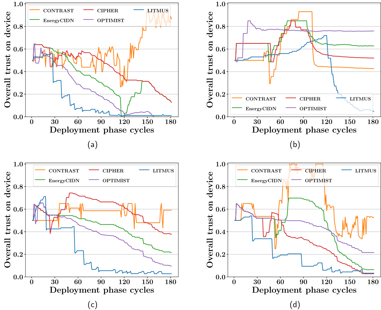
Fig. 12. Attack resiliency of frameworks that use trust management. (a) Trust penalty for inconsistency attacks. (b) Trust penalty for betrayal attacks. (c) Trust penalty for newcomer attacks. (d) Trust penalty for mimicry attacks.
