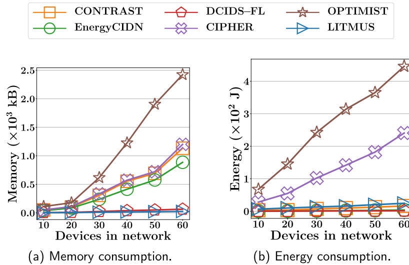
Fig. 11. Memory and energy consumption of the frameworks during attacks against network size.
