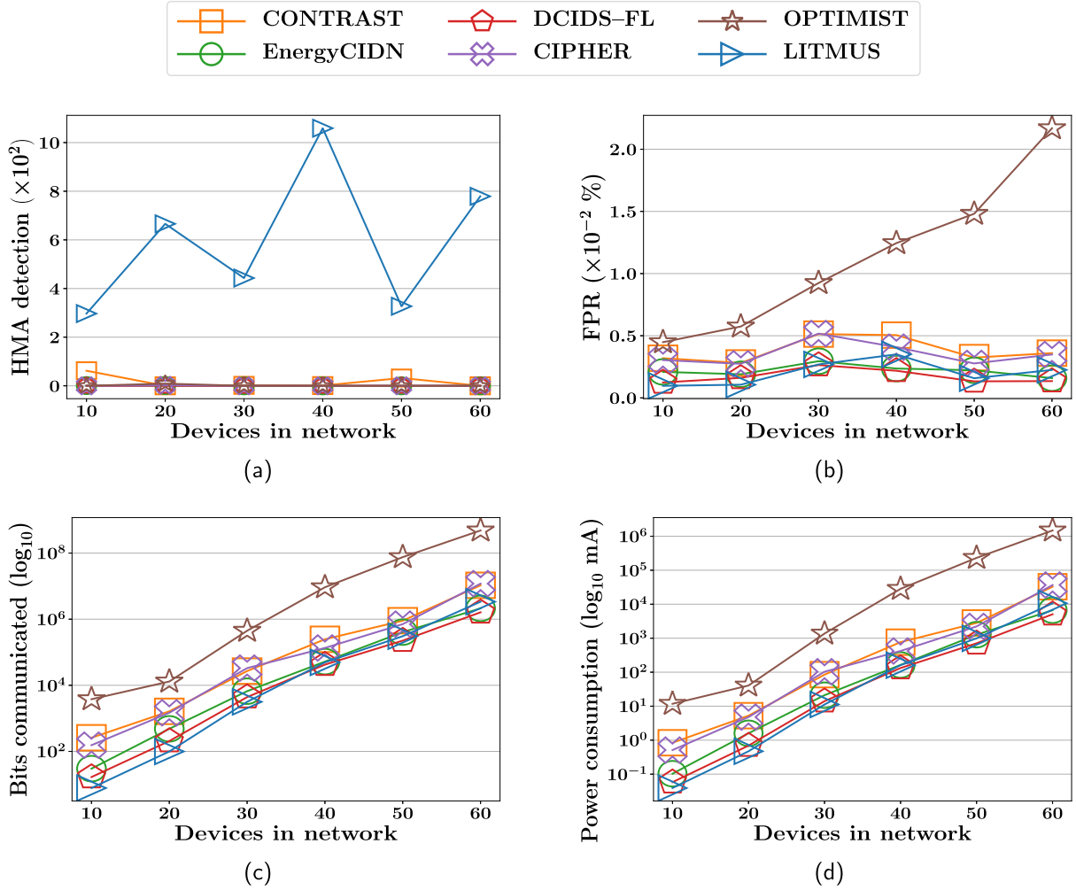
Fig. 8. Results for HMA detection against network size. (a) HMA detection rate. (b) False positive rate. (c) Payload bits communicated. (d) Energy consumption in communication.
