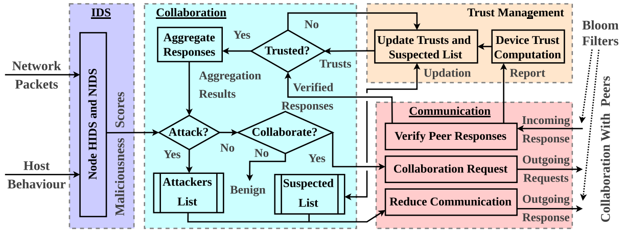
Fig. 2. Schematic view of the modules of LITMUS.
