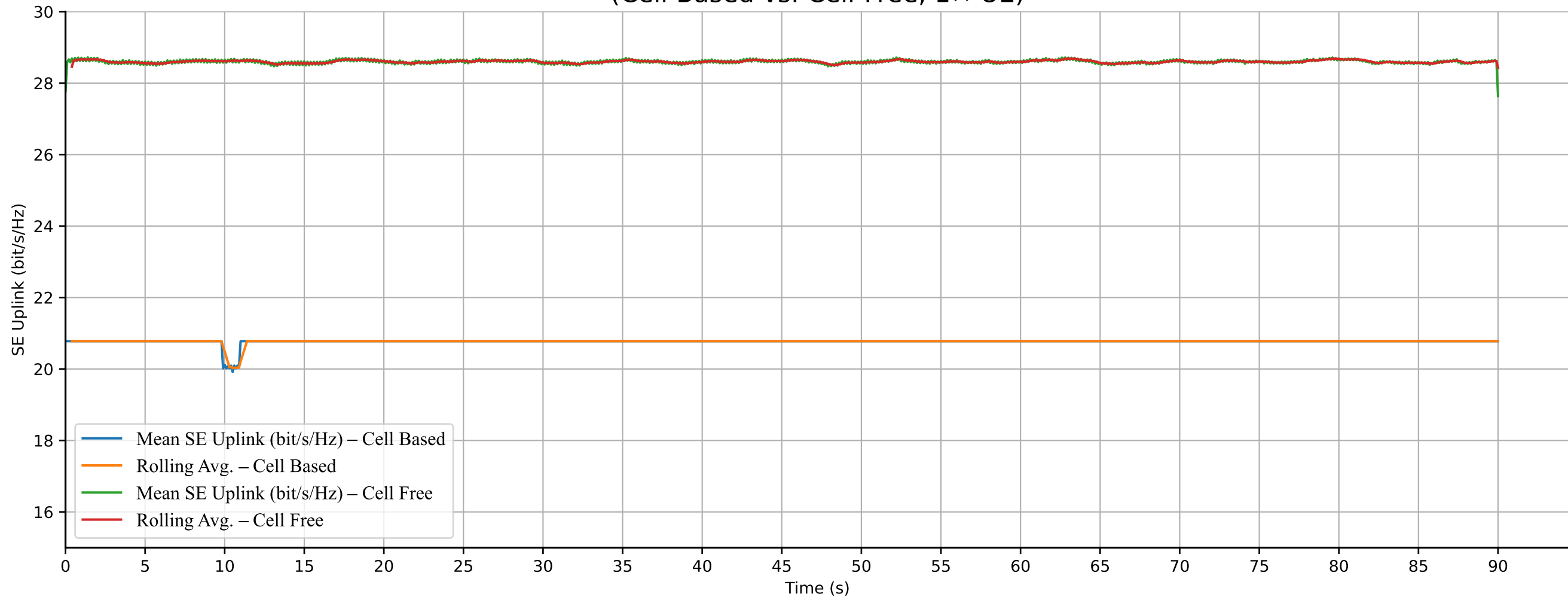
Mean SE per Time (Uplink) (Cell-Based vs. Cell-Free, 1× UE)
