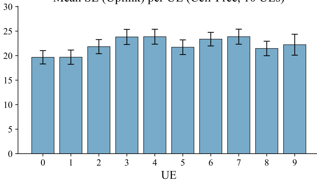
Mean SE (Uplink) per UE (Cell-Free, 10 UEs)
