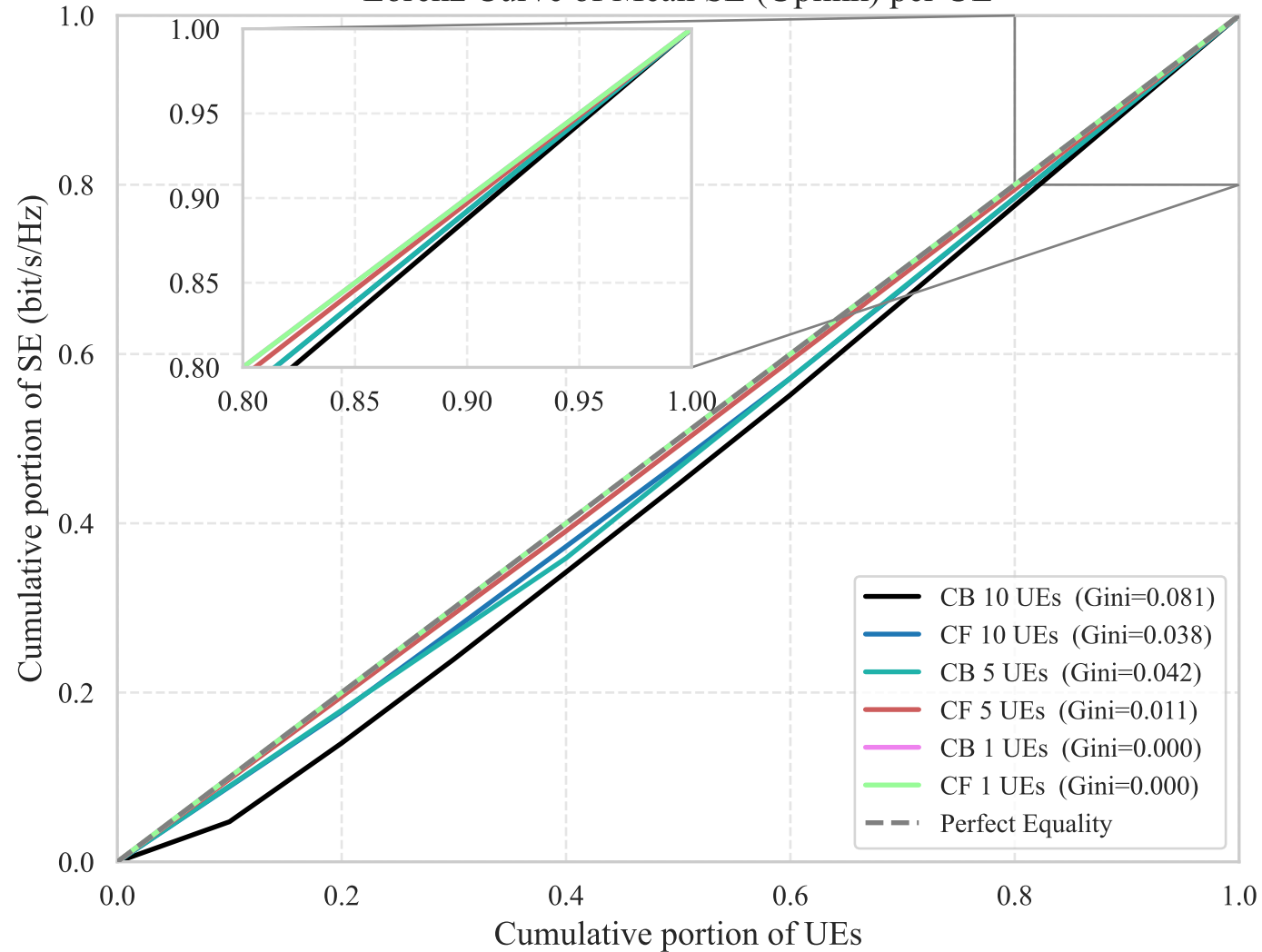
Lorenz Curve of Mean SE (Uplink) per UE
