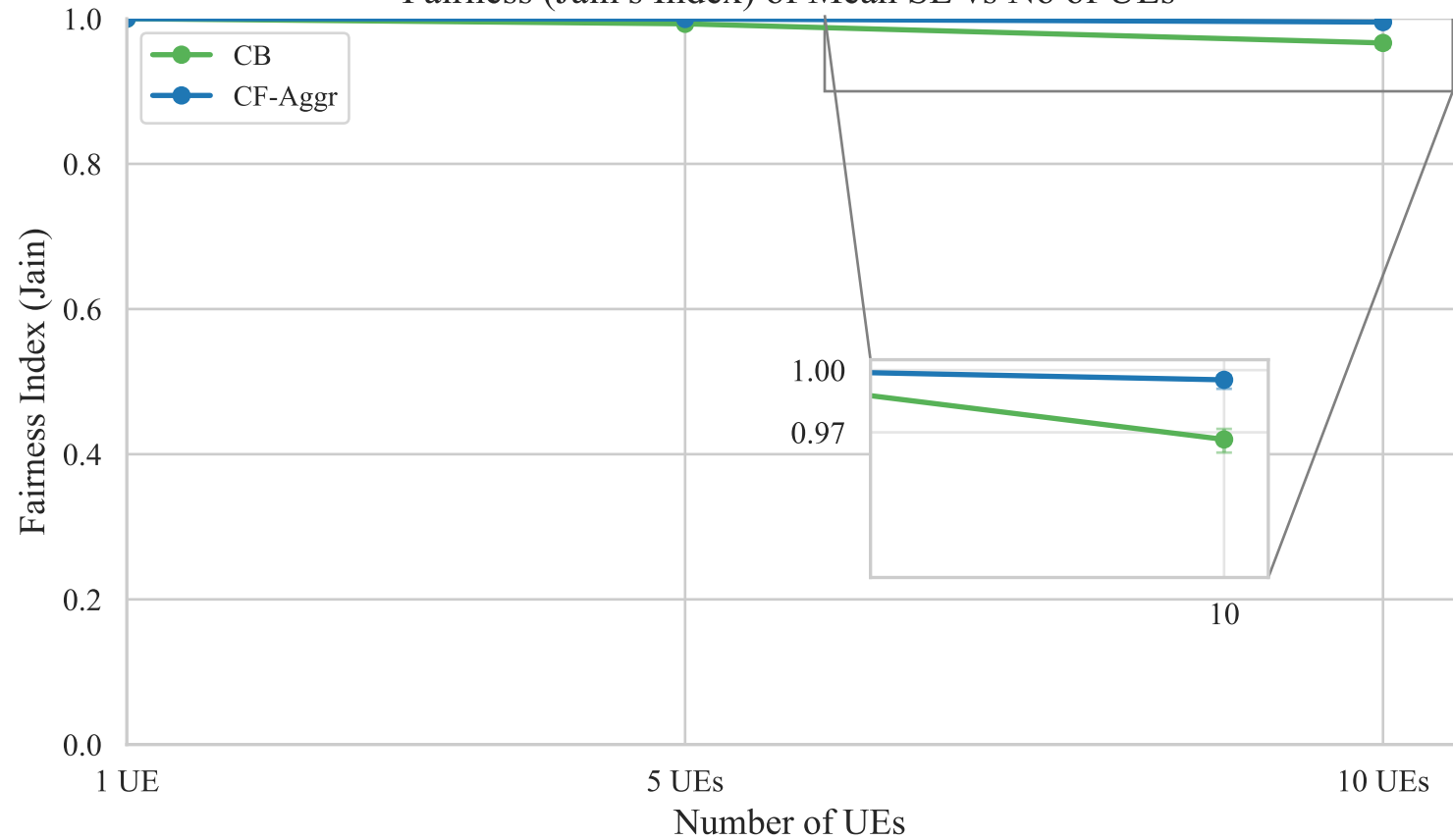
Fairness (Jain's Index) of Mean SE vs No of UEs
