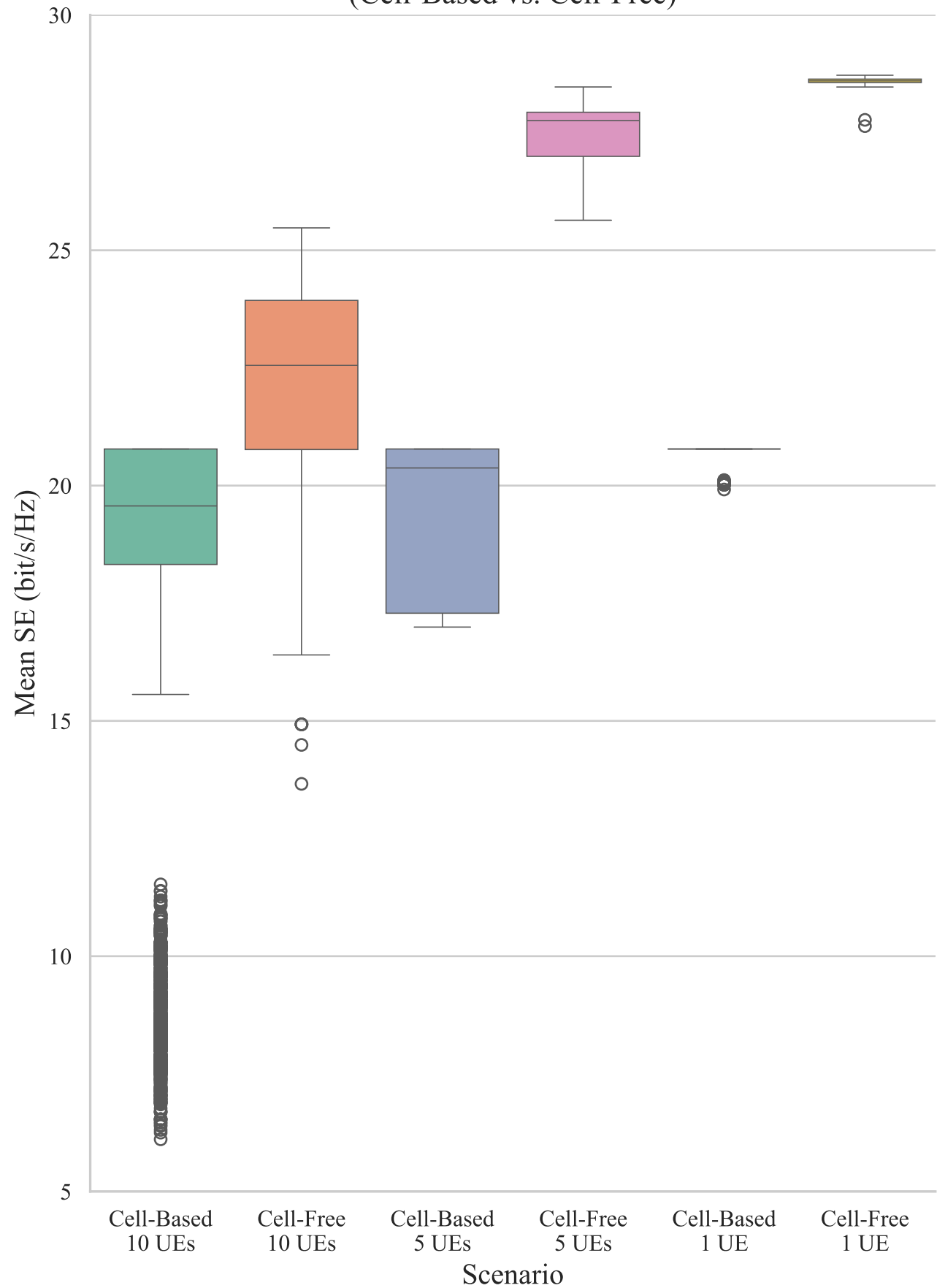
Distribution of Mean SE (Uplink) per Scenario (Cell-Based vs. Cell-Free)
