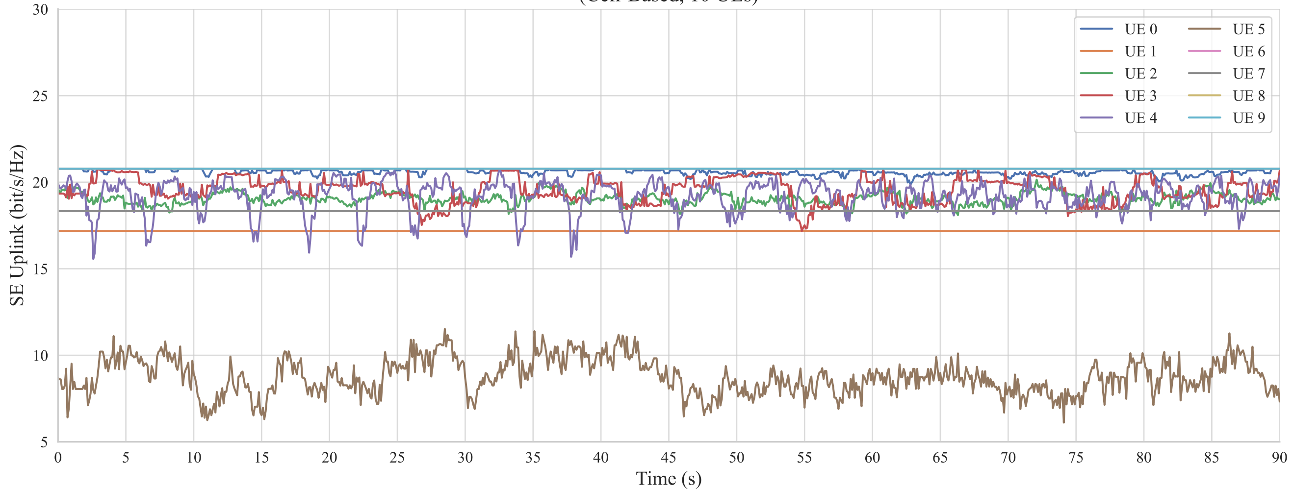
Mean SE per Time (Uplink) (Cell-Based, 10 UEs)
