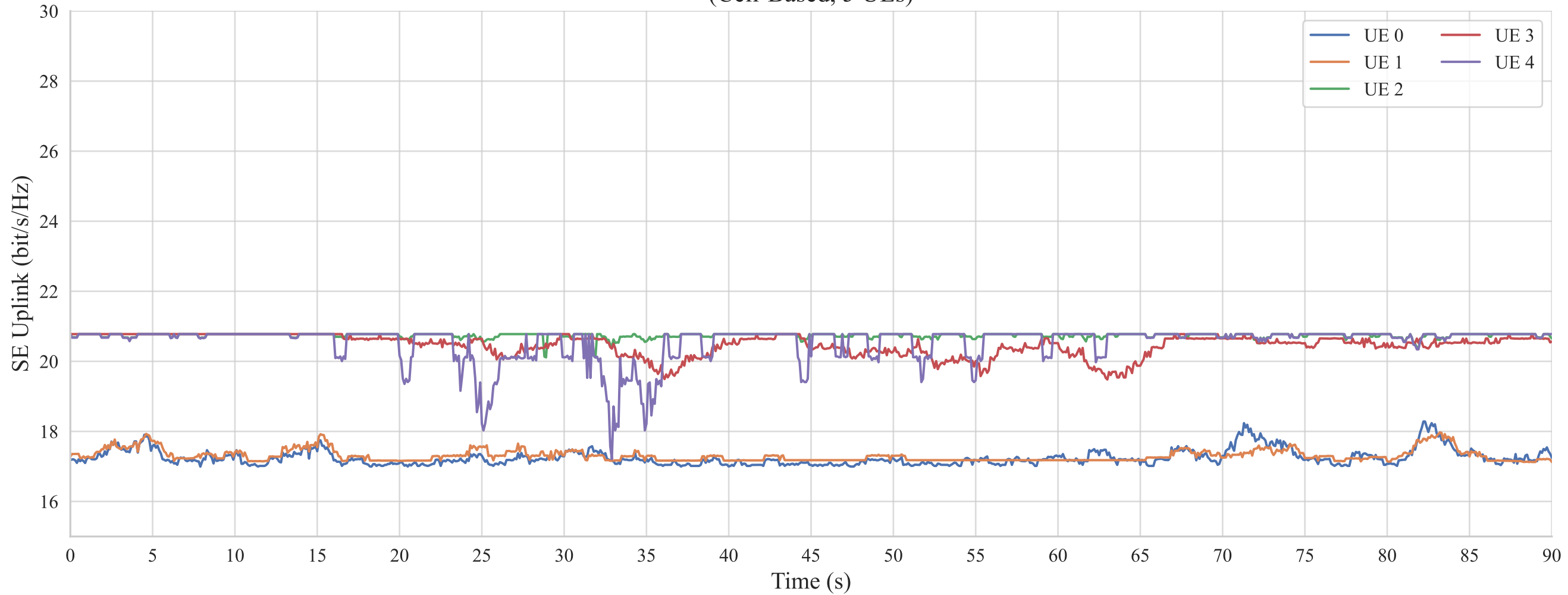
Mean SE per Time (Uplink) (Cell-Based, 5 UEs)
