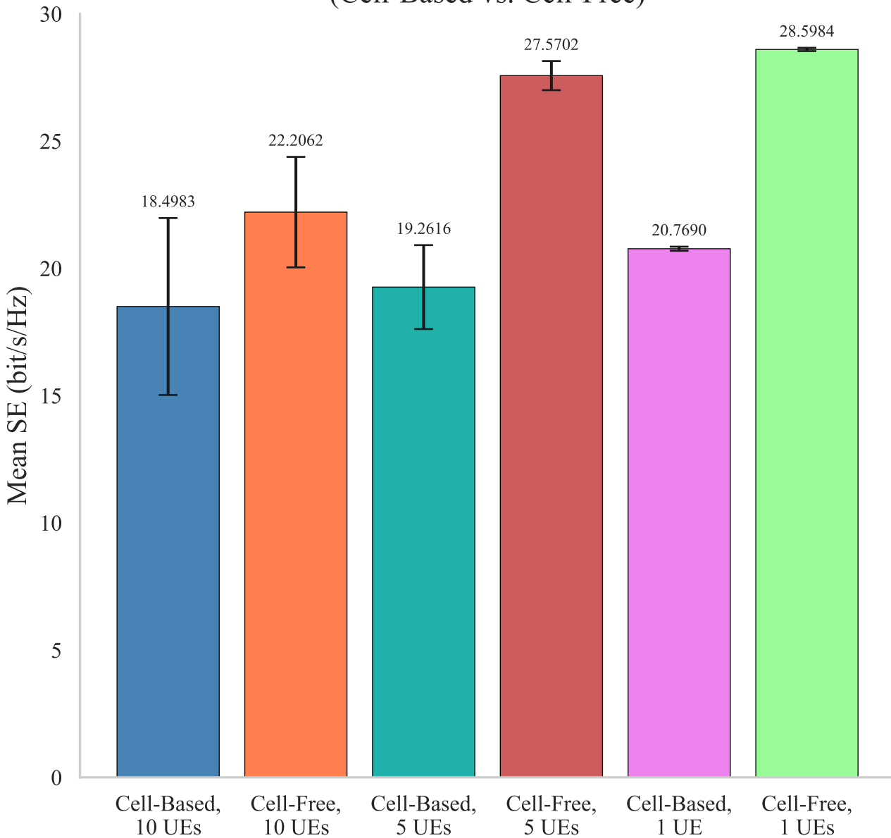
Mean SE per Scenario (Uplink) (Cell-Based vs. Cell-Free)
