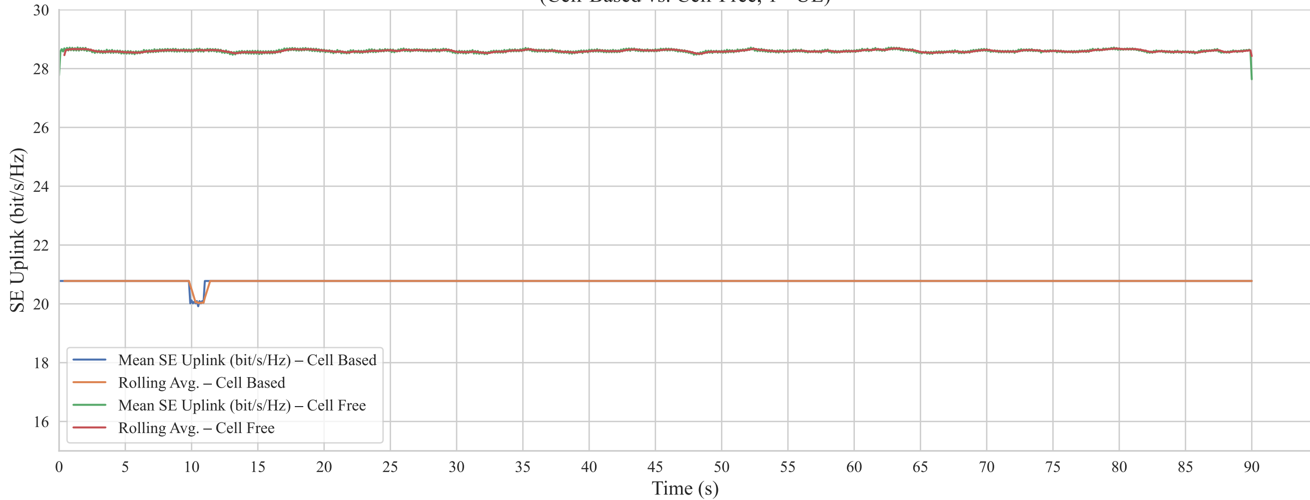
Mean SE per Time (Uplink) (Cell-Based vs. Cell-Free, 1 \times UE)
