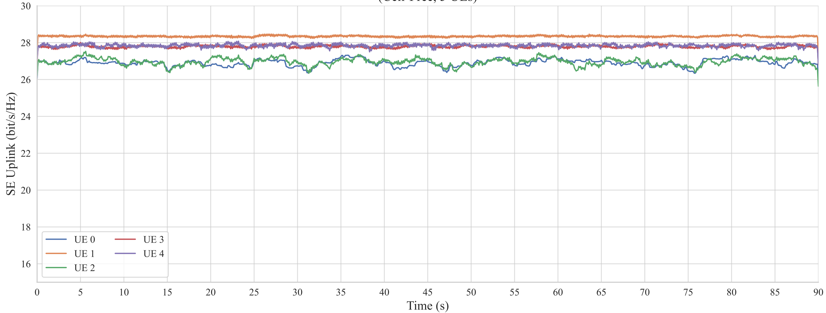
Mean SE per Time (Uplink) (Cell-Free, 5 UEs)
