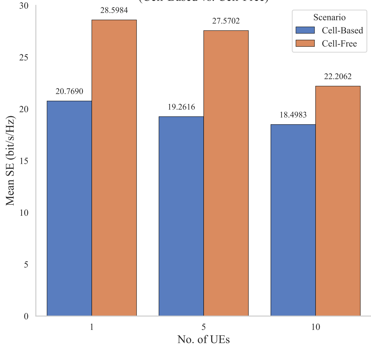
SE per UE (Uplink) (Cell-Based vs. Cell-Free)
