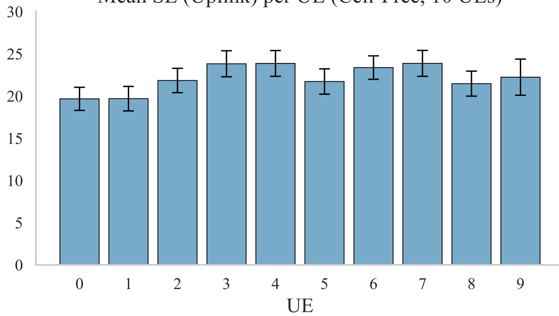
Mean SE (Uplink) per UE (Cell-Free, 10 UEs)
