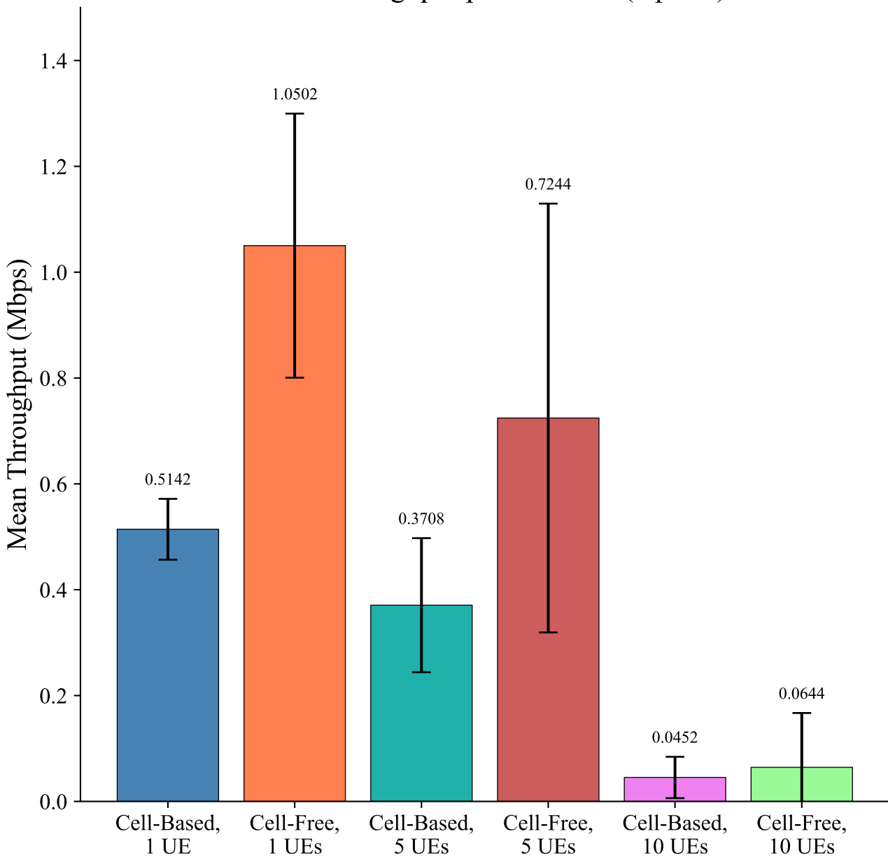
Mean Throughput per Scenario (Uplink)
